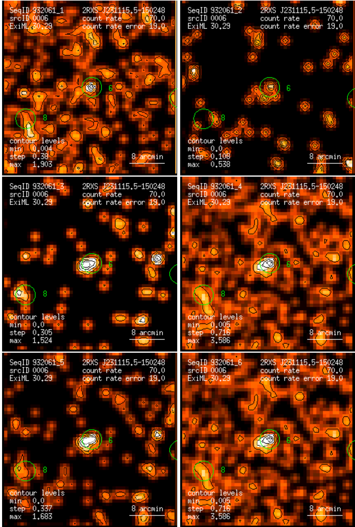
Figure 6: RASS 932061: detection 0006: band rate images, Gaussian filter: (1) PSPC channels 11 – 41, (2) 52 – 90, (3) 91 – 201, (4) 11 – 235, (5) 52 – 201, (6) 11 – 201. Broad band rates in counts/ks. Band rate contour levels in counts/ks/arcmin 2 .
