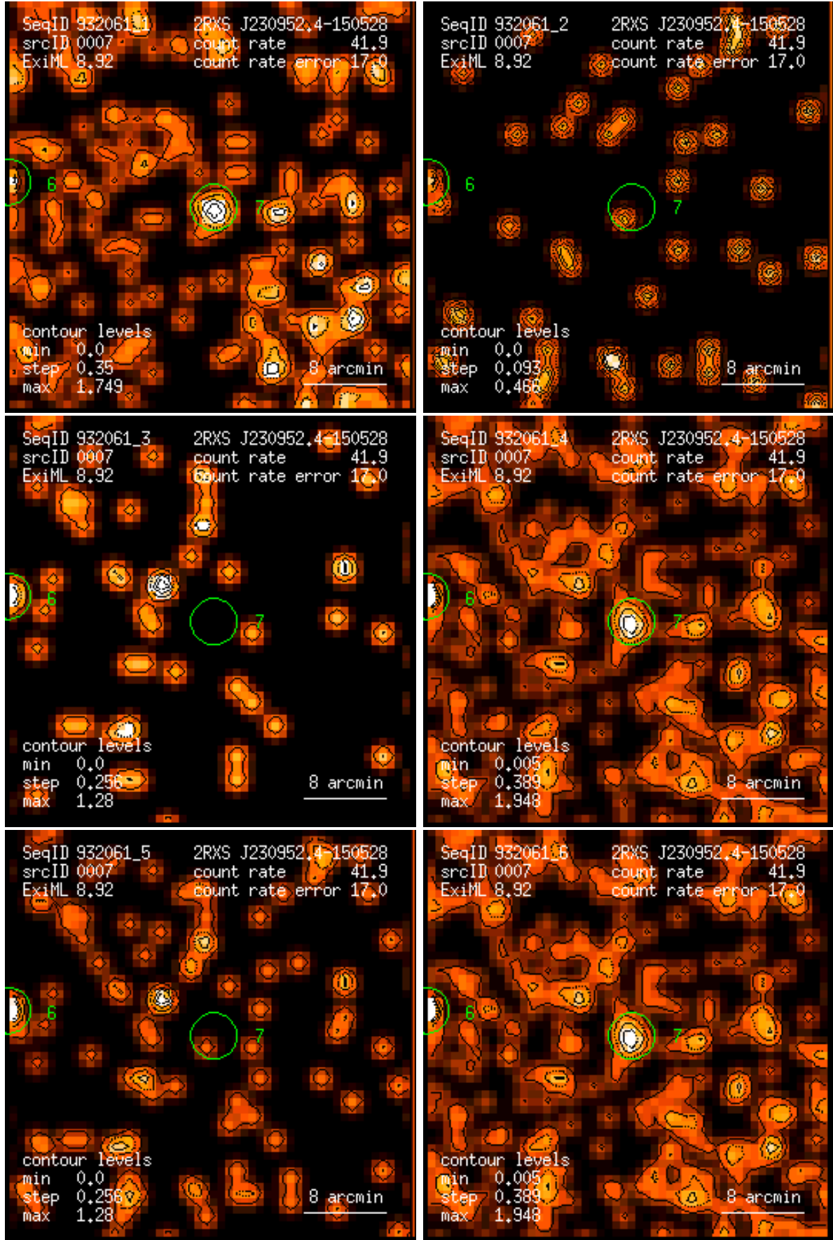
Figure 7: RASS 932061: detection 0007: band rate images, Gaussian filter: (1) PSPC channels 11 – 41, (2) 52 – 90, (3) 91 – 201, (4) 11 – 235, (5) 52 – 201, (6) 11 – 201. Broad band rates in counts/ks. Band rate contour levels in counts/ks/arcmin 2 .
