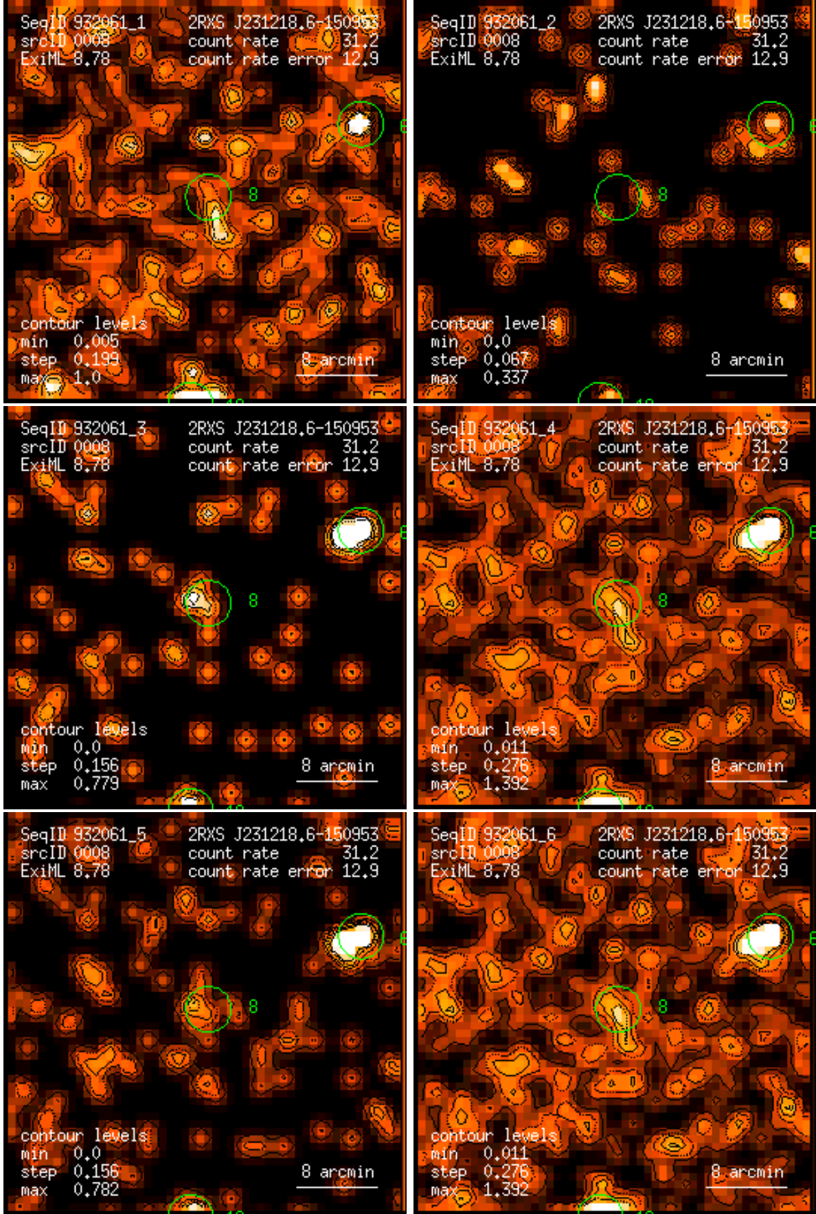
Figure 8: RASS 932061: detection 0008: band rate images, Gaussian filter: (1) PSPC channels 11 – 41, (2) 52 – 90, (3) 91 – 201, (4) 11 – 235, (5) 52 – 201, (6) 11 – 201. Broad band rates in counts/ks. Band rate contour levels in counts/ks/arcmin 2 .
