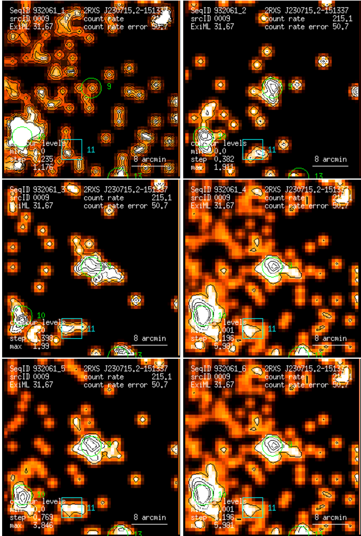
Figure 9: RASS 932061: detection 0009: band rate images, Gaussian filter: (1) PSPC channels 11 – 41, (2) 52 – 90, (3) 91 – 201, (4) 11 – 235, (5) 52 – 201, (6) 11 – 201. Broad band rates in counts/ks. Band rate contour levels in counts/ks/arcmin 2 .
