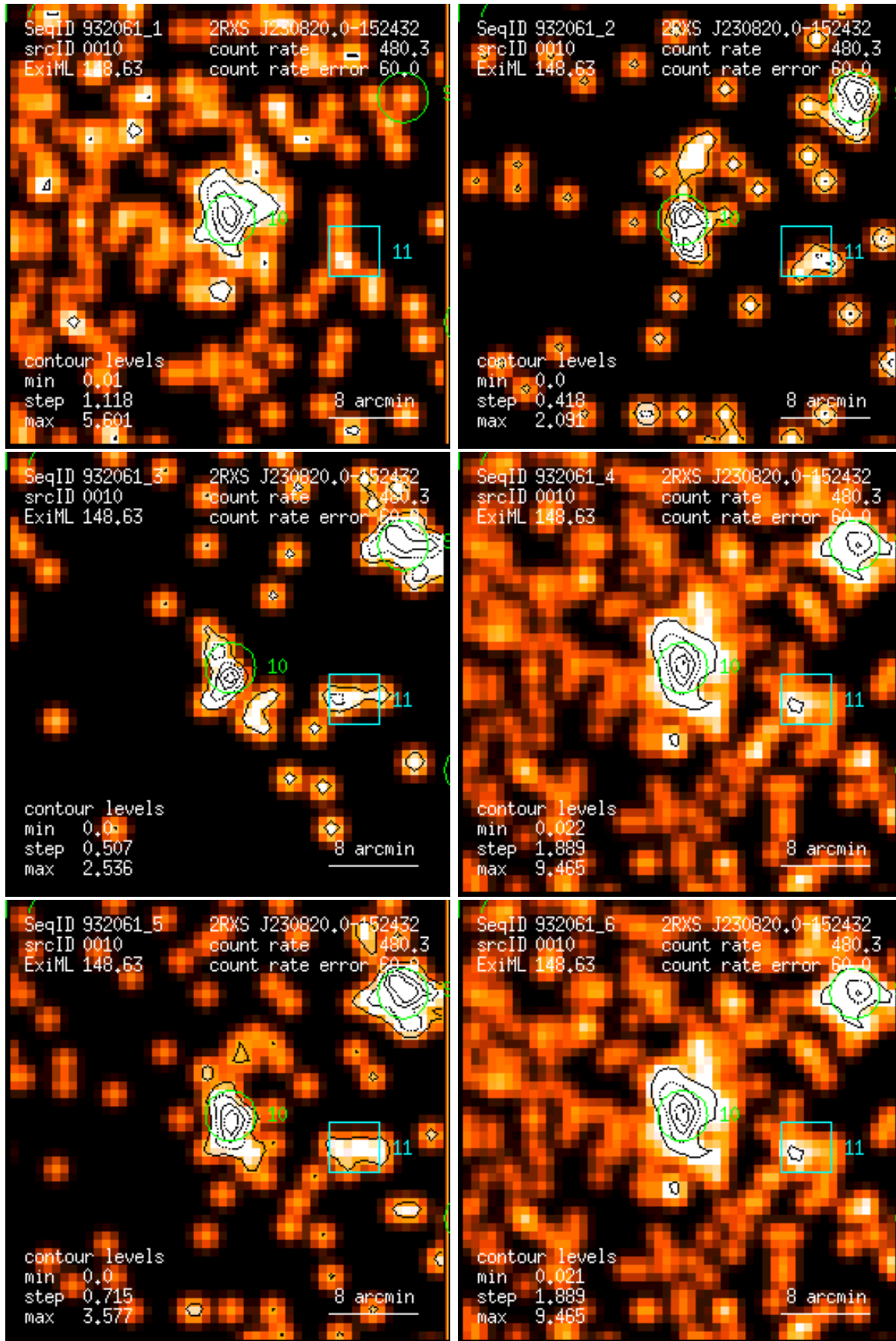
Figure 10: RASS 932061: detection 0010: band rate images, Gaussian filter: (1) PSPC channels 11 – 41, (2) 52 – 90, (3) 91 – 201, (4) 11 – 235, (5) 52 – 201, (6) 11 – 201. Broad band rates in counts/ks. Band rate contour levels in counts/ks/arcmin 2 .
