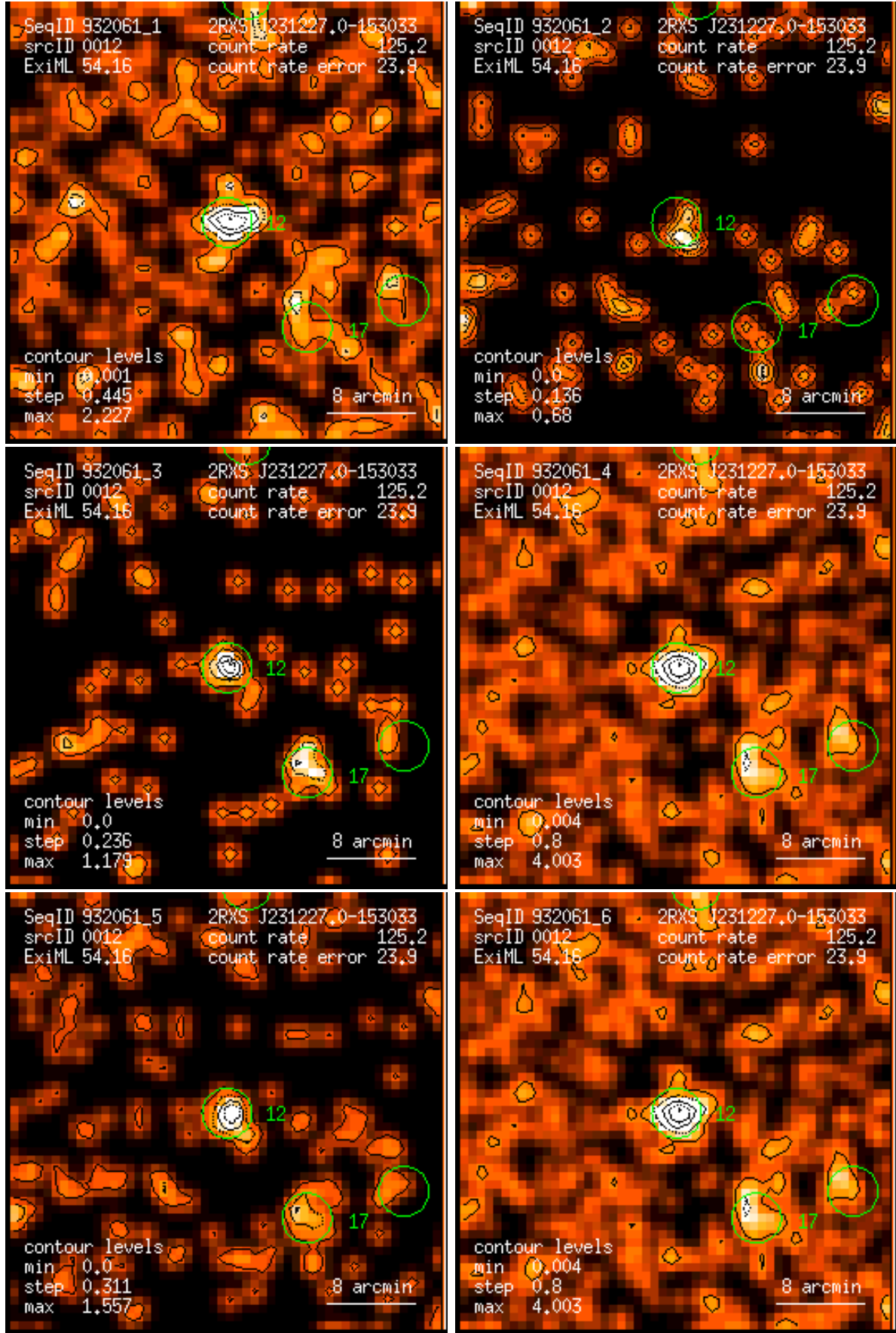
Figure 12: RASS 932061: detection 0012: band rate images, Gaussian filter: (1) PSPC channels 11 – 41, (2) 52 – 90, (3) 91 – 201, (4) 11 – 235, (5) 52 – 201, (6) 11 – 201. Broad band rates in counts/ks. Band rate contour levels in counts/ks/arcmin 2 .
