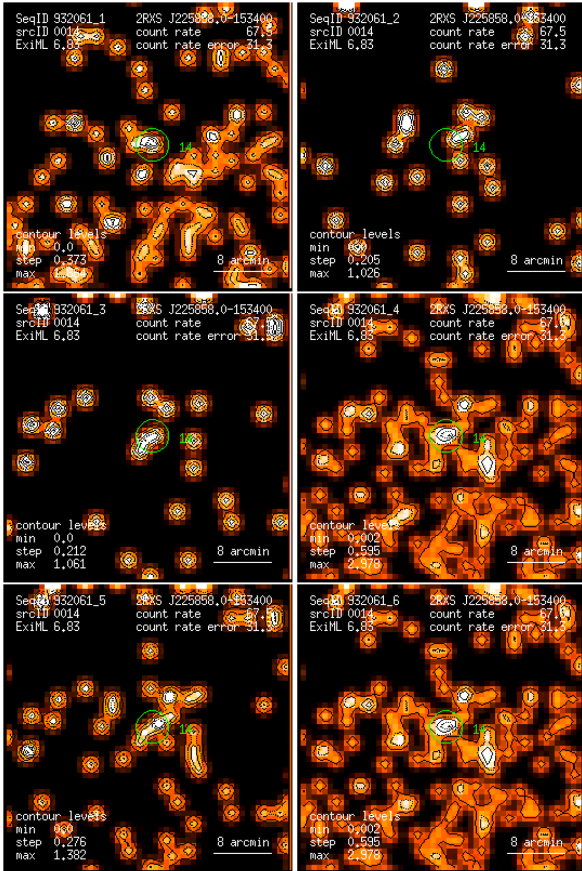
Figure 14: RASS 932061: detection 0014: band rate images, Gaussian filter: (1) PSPC channels 11 – 41, (2) 52 – 90, (3) 91 – 201, (4) 11 – 235, (5) 52 – 201, (6) 11 – 201. Broad band rates in counts/ks. Band rate contour levels in counts/ks/arcmin 2 .
