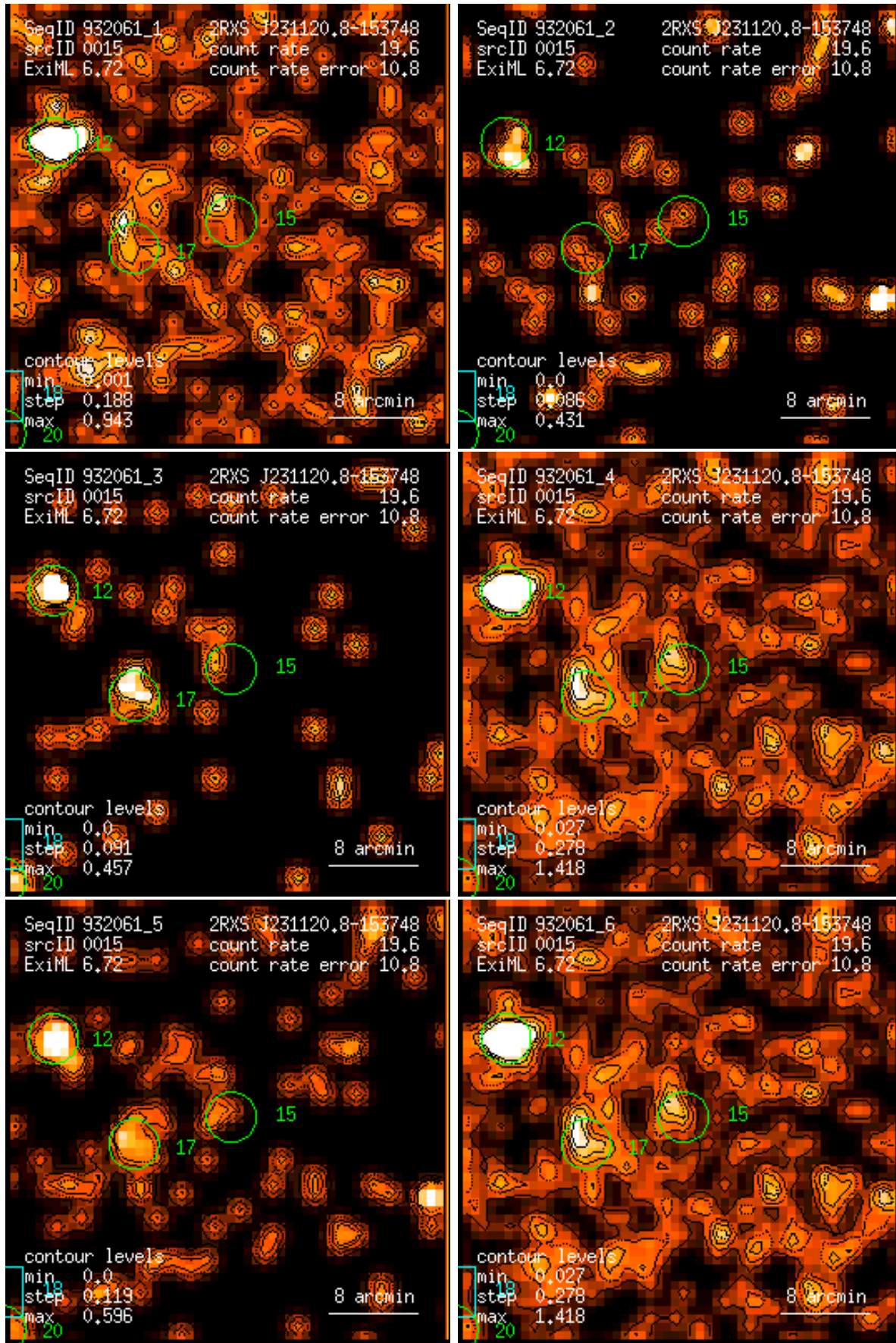
Figure 15: RASS 932061: detection 0015: band rate images, Gaussian filter: (1) PSPC channels 11 – 41, (2) 52 – 90, (3) 91 – 201, (4) 11 – 235, (5) 52 – 201, (6) 11 – 201. Broad band rates in counts/ks. Band rate contour levels in counts/ks/arcmin 2 .
