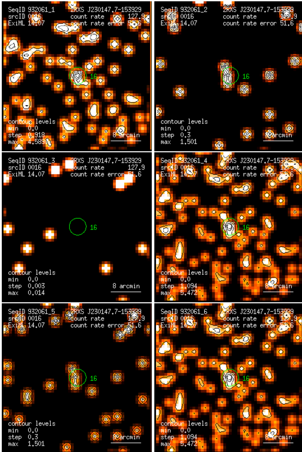
Figure 16: RASS 932061: detection 0016: band rate images, Gaussian filter: (1) PSPC channels 11 – 41, (2) 52 – 90, (3) 91 – 201, (4) 11 – 235, (5) 52 – 201, (6) 11 – 201. Broad band rates in counts/ks. Band rate contour levels in counts/ks/arcmin 2 .
