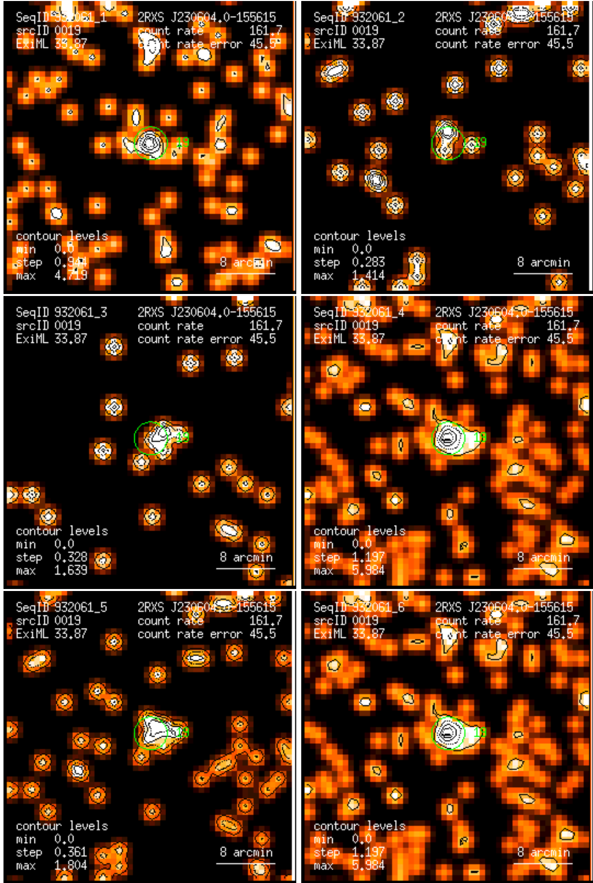
Figure 19: RASS 932061: detection 0019: band rate images, Gaussian filter: (1) PSPC channels 11 – 41, (2) 52 – 90, (3) 91 – 201, (4) 11 – 235, (5) 52 – 201, (6) 11 – 201. Broad band rates in counts/ks. Band rate contour levels in counts/ks/arcmin 2 .
