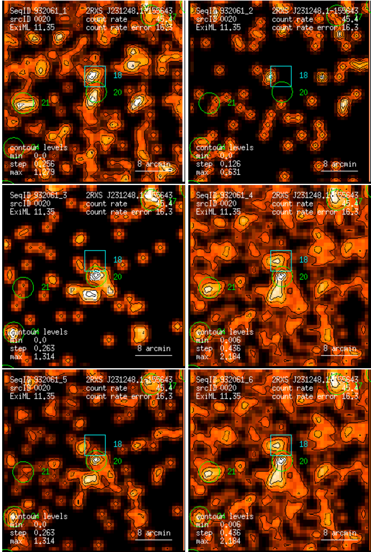
Figure 20: RASS 932061: detection 0020: band rate images, Gaussian filter: (1) PSPC channels 11 – 41, (2) 52 – 90, (3) 91 – 201, (4) 11 – 235, (5) 52 – 201, (6) 11 – 201. Broad band rates in counts/ks. Band rate contour levels in counts/ks/arcmin 2 .
