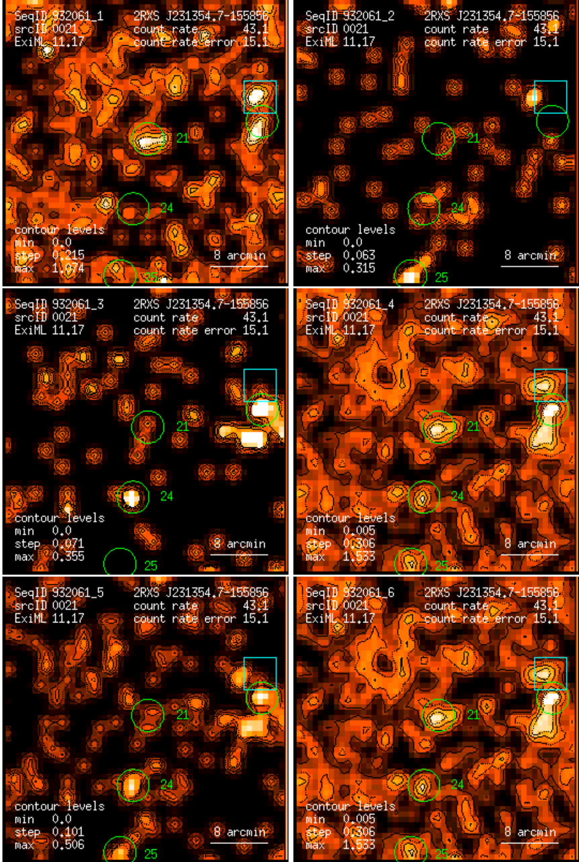
Figure 21: RASS 932061: detection 0021: band rate images, Gaussian filter: (1) PSPC channels 11 – 41, (2) 52 – 90, (3) 91 – 201, (4) 11 – 235, (5) 52 – 201, (6) 11 – 201. Broad band rates in counts/ks. Band rate contour levels in counts/ks/arcmin 2 .
