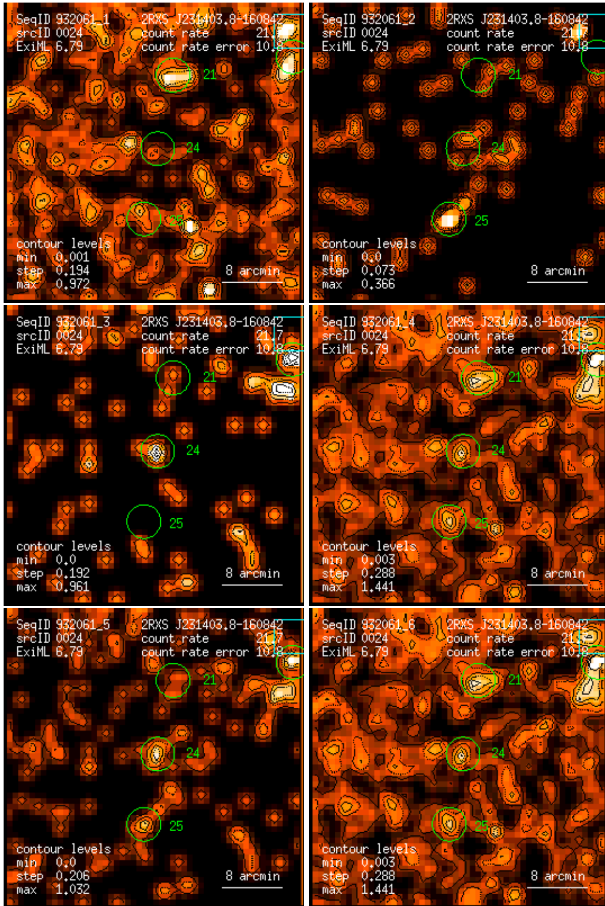
Figure 24: RASS 932061: detection 0024: band rate images, Gaussian filter: (1) PSPC channels 11 – 41, (2) 52 – 90, (3) 91 – 201, (4) 11 – 235, (5) 52 – 201, (6) 11 – 201. Broad band rates in counts/ks. Band rate contour levels in counts/ks/arcmin 2 .
