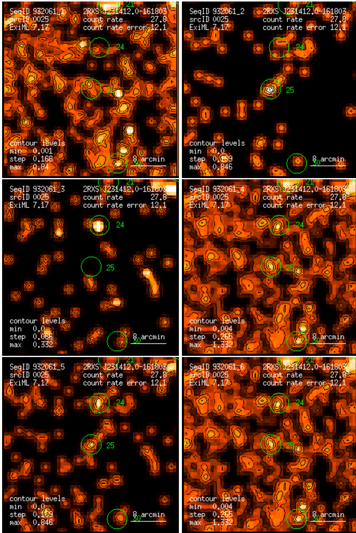
Figure 25: RASS 932061: detection 0025: band rate images, Gaussian filter: (1) PSPC channels 11 – 41, (2) 52 – 90, (3) 91 – 201, (4) 11 – 235, (5) 52 – 201, (6) 11 – 201. Broad band rates in counts/ks. Band rate contour levels in counts/ks/arcmin 2 .
