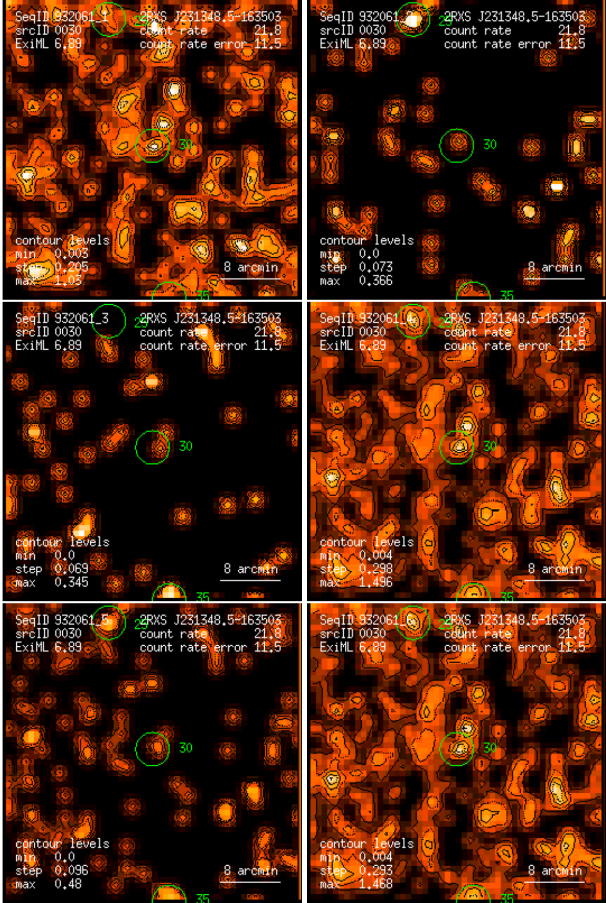
Figure 30: RASS 932061: detection 0030: band rate images, Gaussian filter: (1) PSPC channels 11 – 41, (2) 52 – 90, (3) 91 – 201, (4) 11 – 235, (5) 52 – 201, (6) 11 – 201. Broad band rates in counts/ks. Band rate contour levels in counts/ks/arcmin 2 .
