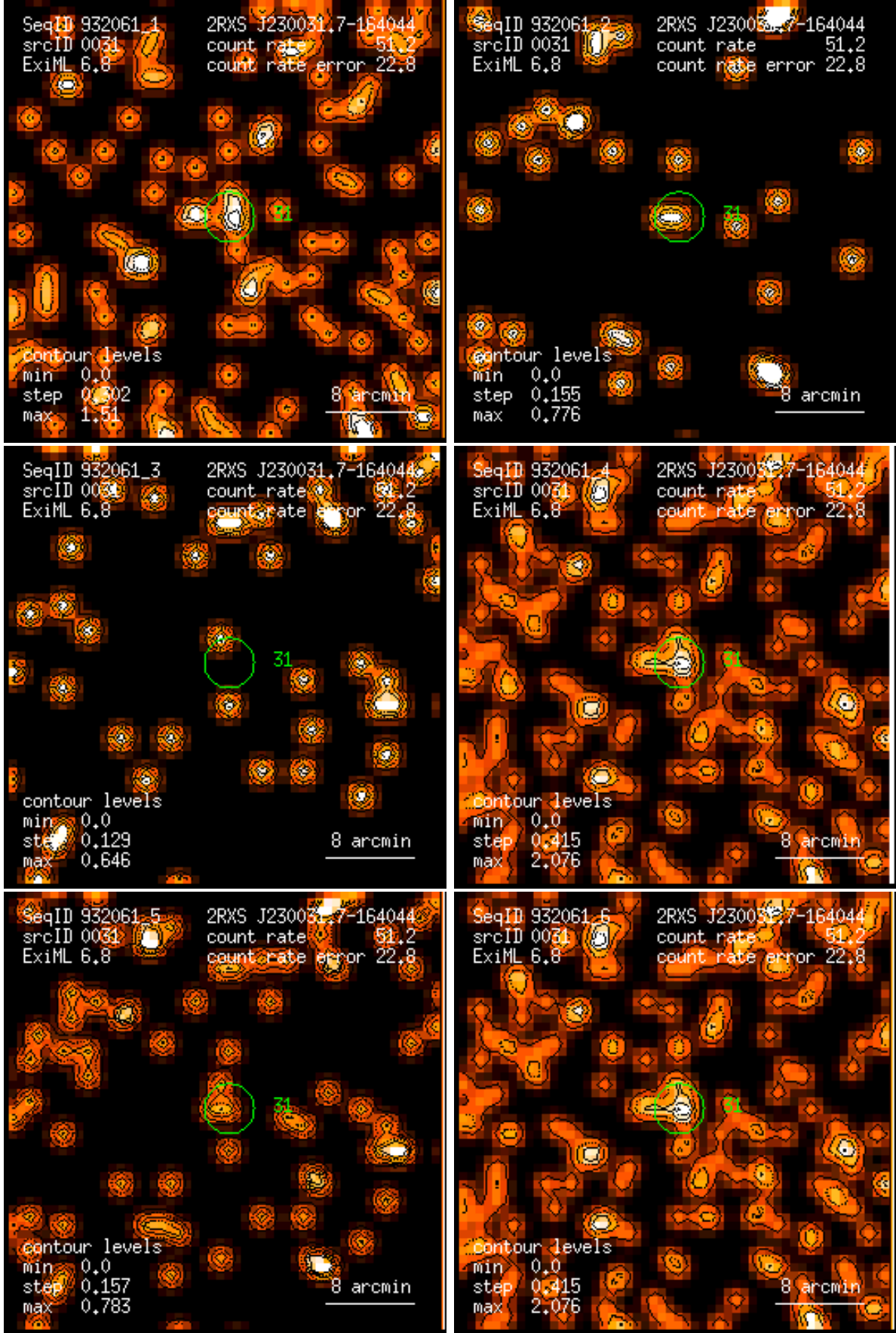
Figure 31: RASS 932061: detection 0031: band rate images, Gaussian filter: (1) PSPC channels 11 – 41, (2) 52 – 90, (3) 91 – 201, (4) 11 – 235, (5) 52 – 201, (6) 11 – 201. Broad band rates in counts/ks. Band rate contour levels in counts/ks/arcmin 2 .
