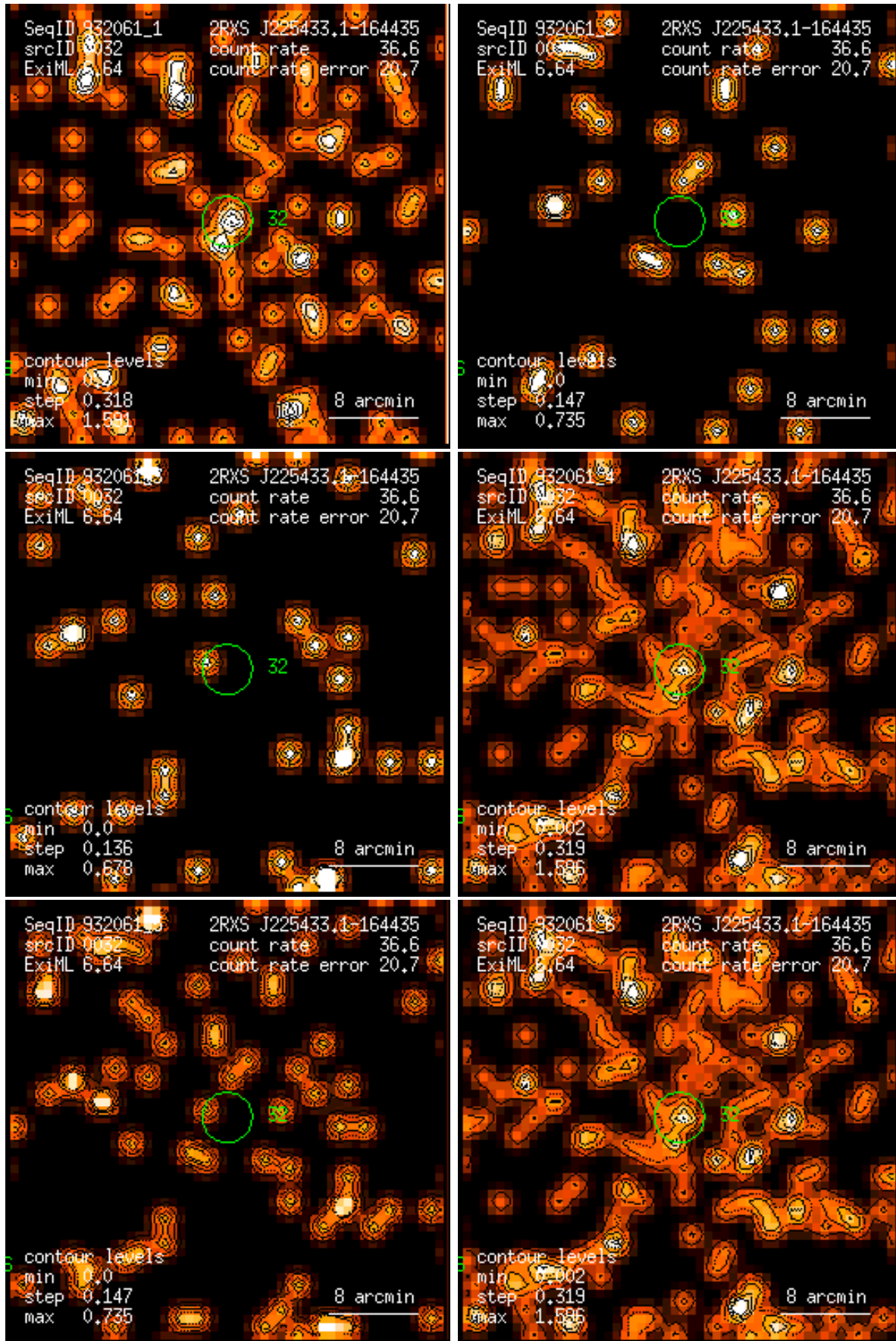
Figure 32: RASS 932061: detection 0032: band rate images, Gaussian filter: (1) PSPC channels 11 – 41, (2) 52 – 90, (3) 91 – 201, (4) 11 – 235, (5) 52 – 201, (6) 11 – 201. Broad band rates in counts/ks. Band rate contour levels in counts/ks/arcmin 2 .
