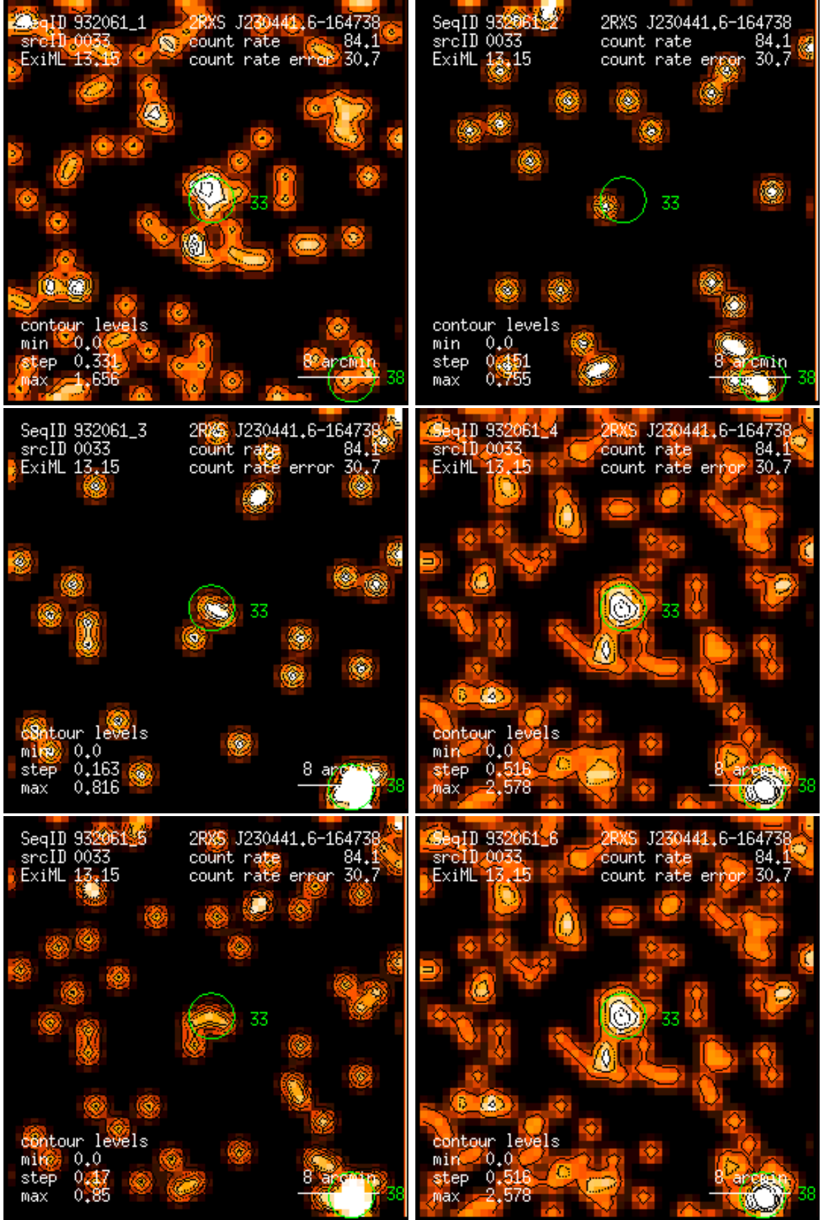
Figure 33: RASS 932061: detection 0033: band rate images, Gaussian filter: (1) PSPC channels 11 – 41, (2) 52 – 90, (3) 91 – 201, (4) 11 – 235, (5) 52 – 201, (6) 11 – 201. Broad band rates in counts/ks. Band rate contour levels in counts/ks/arcmin 2 .
