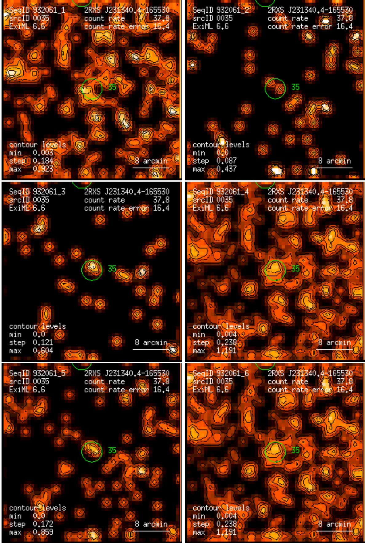
Figure 35: RASS 932061: detection 0035: band rate images, Gaussian filter: (1) PSPC channels 11 – 41, (2) 52 – 90, (3) 91 – 201, (4) 11 – 235, (5) 52 – 201, (6) 11 – 201. Broad band rates in counts/ks. Band rate contour levels in counts/ks/arcmin 2 .
