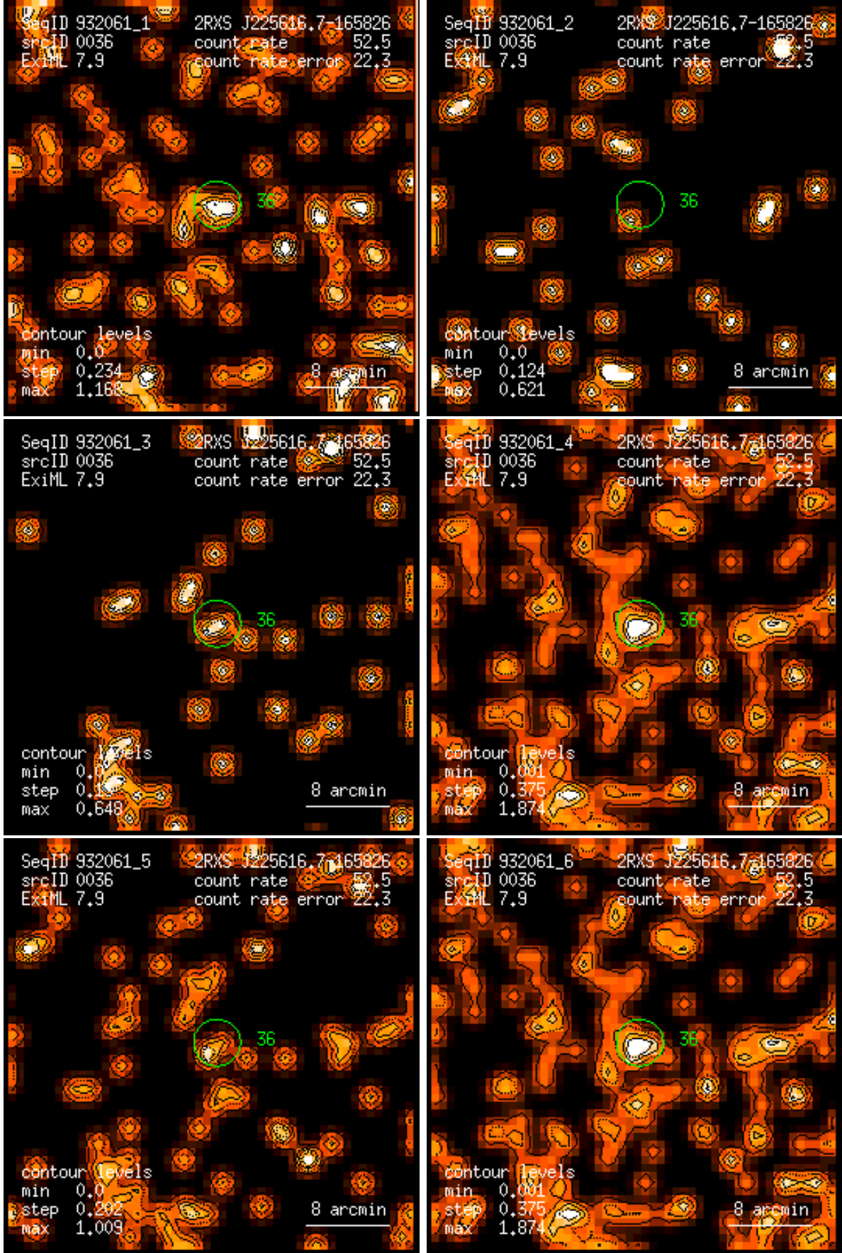
Figure 36: RASS 932061: detection 0036: band rate images, Gaussian filter: (1) PSPC channels 11 – 41, (2) 52 – 90, (3) 91 – 201, (4) 11 – 235, (5) 52 – 201, (6) 11 – 201. Broad band rates in counts/ks. Band rate contour levels in counts/ks/arcmin 2 .
