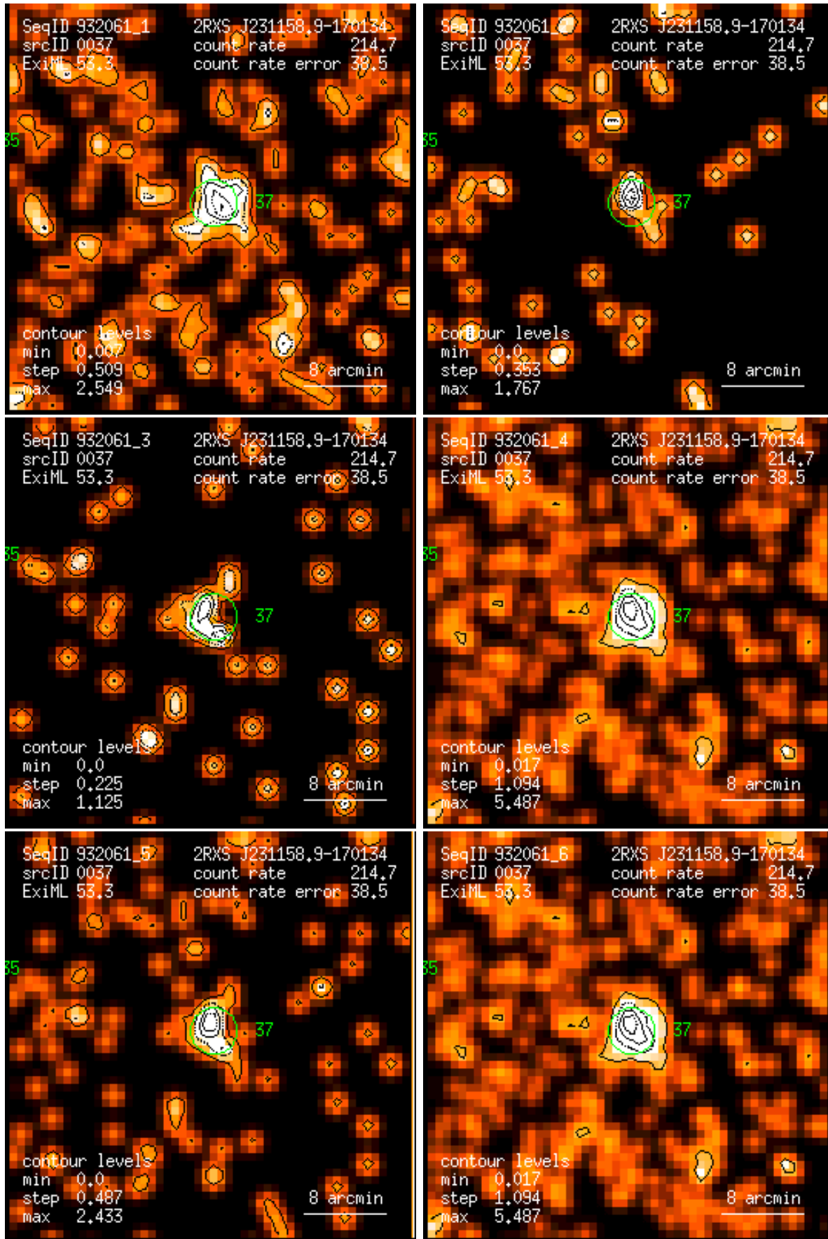
Figure 37: RASS 932061: detection 0037: band rate images, Gaussian filter: (1) PSPC channels 11 – 41, (2) 52 – 90, (3) 91 – 201, (4) 11 – 235, (5) 52 – 201, (6) 11 – 201. Broad band rates in counts/ks. Band rate contour levels in counts/ks/arcmin 2 .
