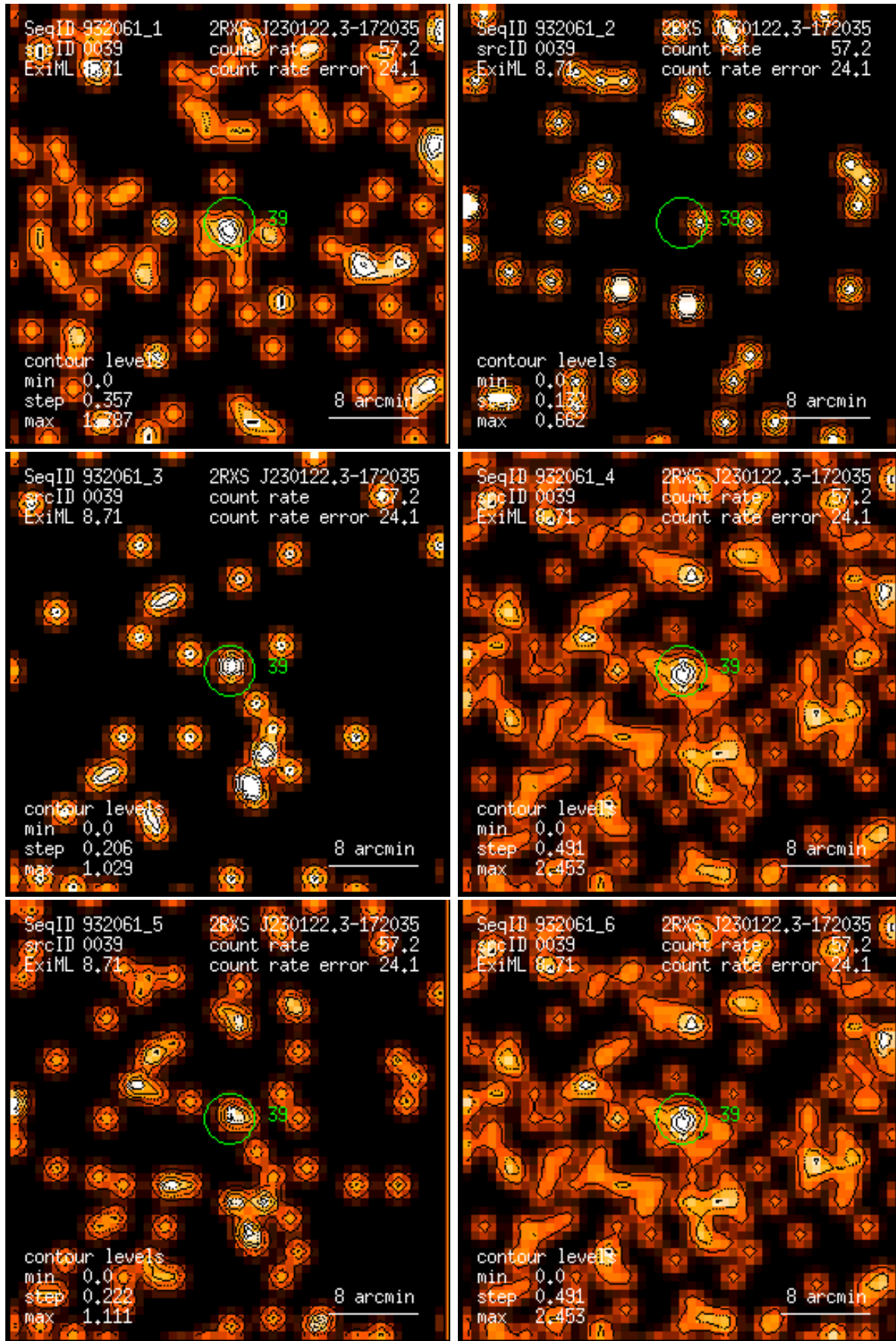
Figure 39: RASS 932061: detection 0039: band rate images, Gaussian filter: (1) PSPC channels 11 – 41, (2) 52 – 90, (3) 91 – 201, (4) 11 – 235, (5) 52 – 201, (6) 11 – 201. Broad band rates in counts/ks. Band rate contour levels in counts/ks/arcmin 2 .
