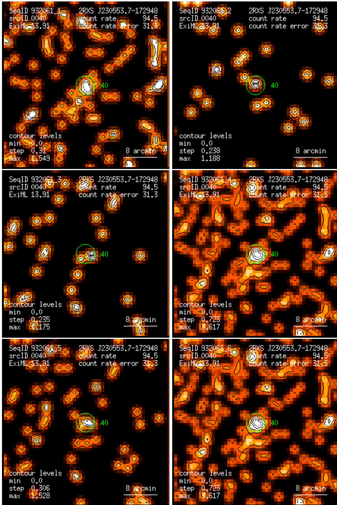
Figure 40: RASS 932061: detection 0040: band rate images, Gaussian filter: (1) PSPC channels 11 – 41, (2) 52 – 90, (3) 91 – 201, (4) 11 – 235, (5) 52 – 201, (6) 11 – 201. Broad band rates in counts/ks. Band rate contour levels in counts/ks/arcmin 2 .
