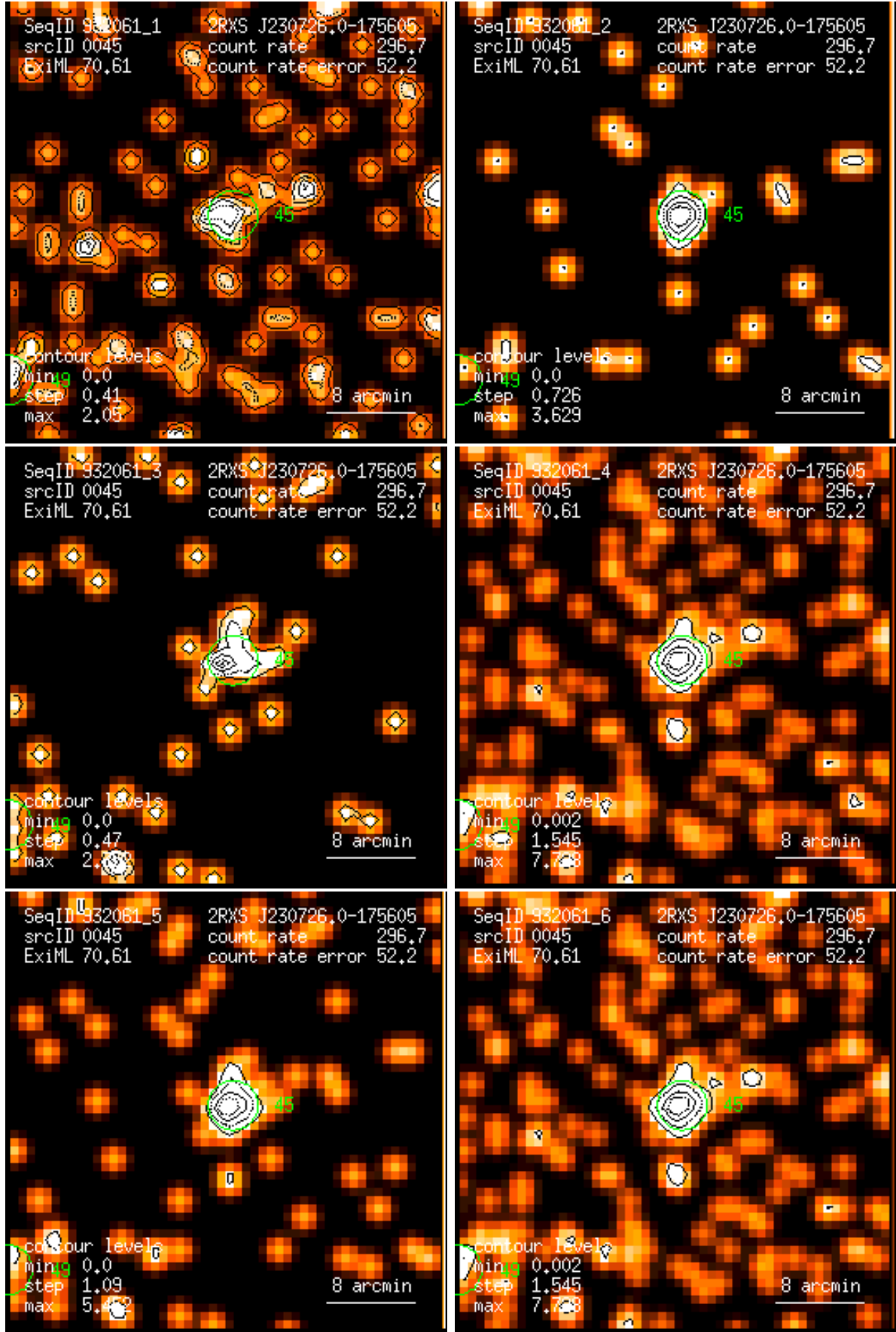
Figure 45: RASS 932061: detection 0045: band rate images, Gaussian filter: (1) PSPC channels 11 – 41, (2) 52 – 90, (3) 91 – 201, (4) 11 – 235, (5) 52 – 201, (6) 11 – 201. Broad band rates in counts/ks. Band rate contour levels in counts/ks/arcmin 2 .
