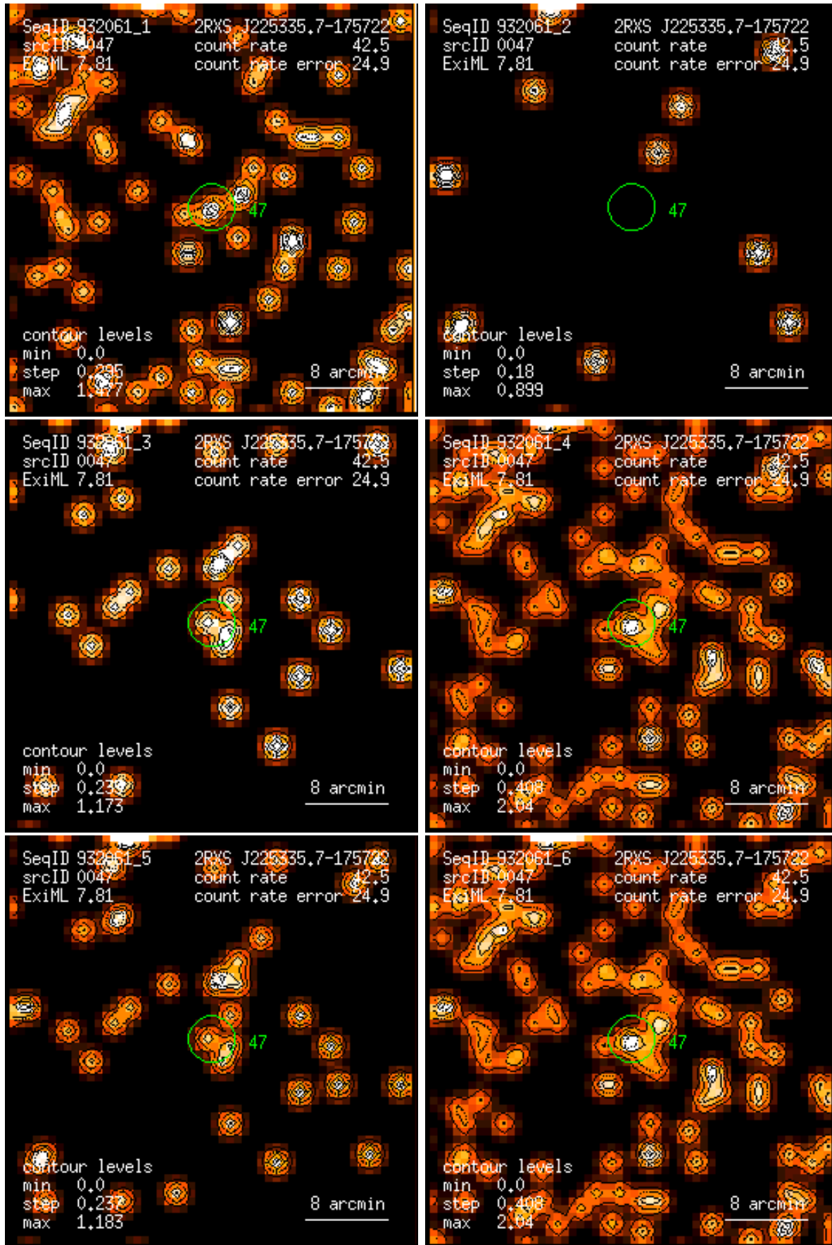
Figure 47: RASS 932061: detection 0047: band rate images, Gaussian filter: (1) PSPC channels 11 – 41, (2) 52 – 90, (3) 91 – 201, (4) 11 – 235, (5) 52 – 201, (6) 11 – 201. Broad band rates in counts/ks. Band rate contour levels in counts/ks/arcmin 2 .
