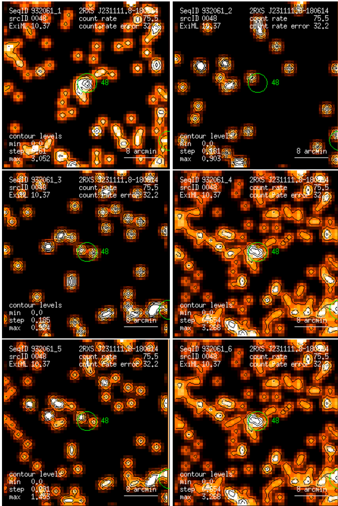
Figure 48: RASS 932061: detection 0048: band rate images, Gaussian filter: (1) PSPC channels 11 – 41, (2) 52 – 90, (3) 91 – 201, (4) 11 – 235, (5) 52 – 201, (6) 11 – 201. Broad band rates in counts/ks. Band rate contour levels in counts/ks/arcmin 2 .
