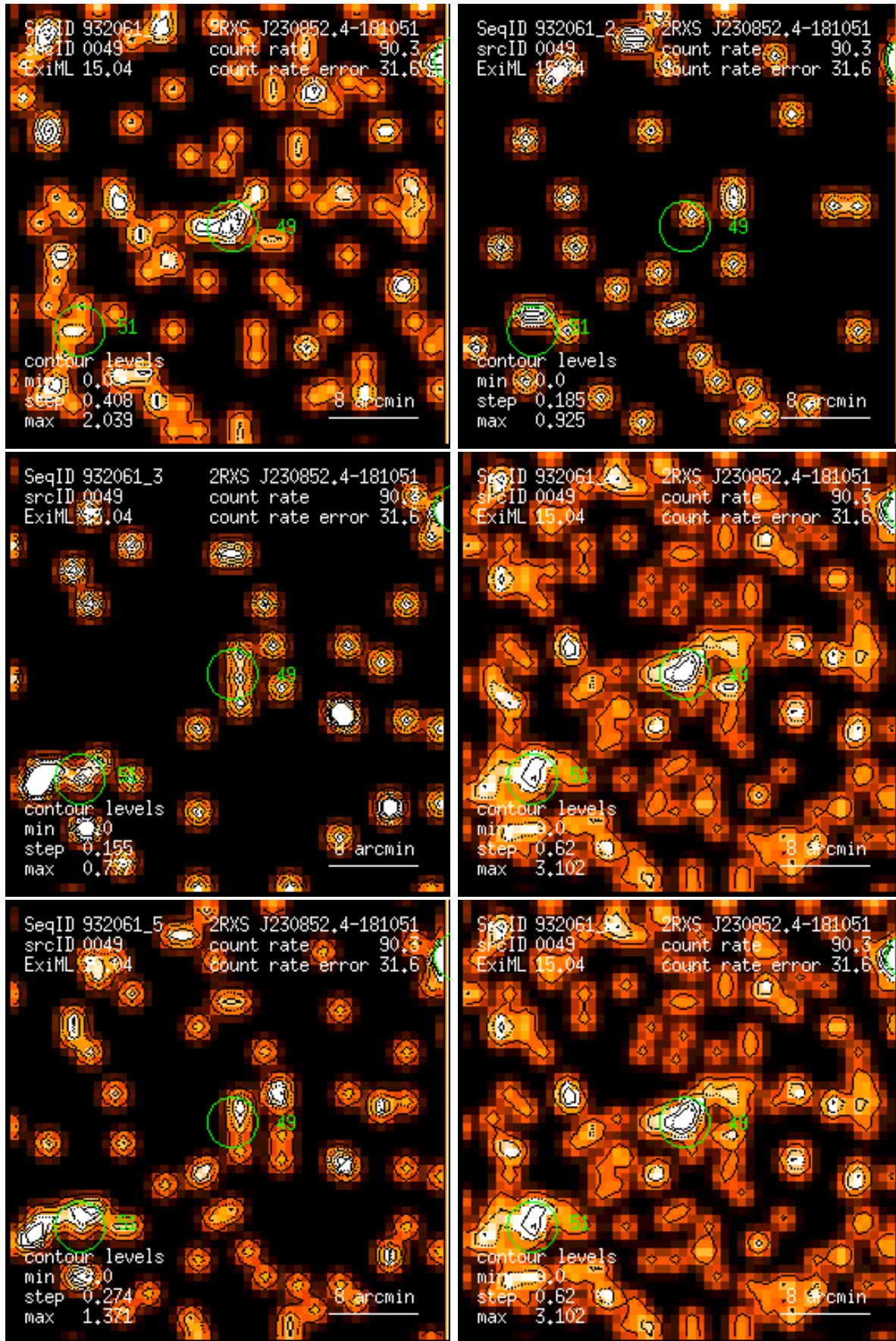
Figure 49: RASS 932061: detection 0049: band rate images, Gaussian filter: (1) PSPC channels 11 – 41, (2) 52 – 90, (3) 91 – 201, (4) 11 – 235, (5) 52 – 201, (6) 11 – 201. Broad band rates in counts/ks. Band rate contour levels in counts/ks/arcmin 2 .
