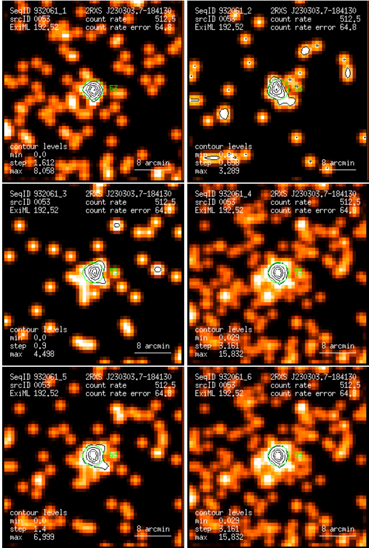
Figure 53: RASS 932061: detection 0053: band rate images, Gaussian filter: (1) PSPC channels 11 – 41, (2) 52 – 90, (3) 91 – 201, (4) 11 – 235, (5) 52 – 201, (6) 11 – 201. Broad band rates in counts/ks. Band rate contour levels in counts/ks/arcmin 2 .
