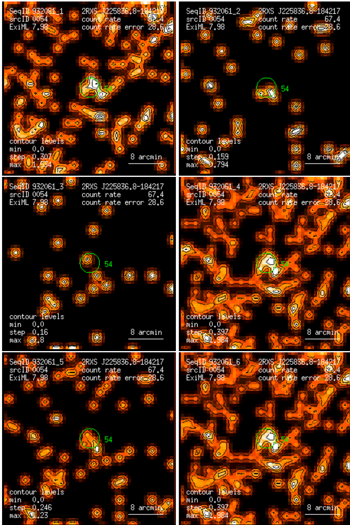
Figure 54: RASS 932061: detection 0054: band rate images, Gaussian filter: (1) PSPC channels 11 – 41, (2) 52 – 90, (3) 91 – 201, (4) 11 – 235, (5) 52 – 201, (6) 11 – 201. Broad band rates in counts/ks. Band rate contour levels in counts/ks/arcmin 2 .
