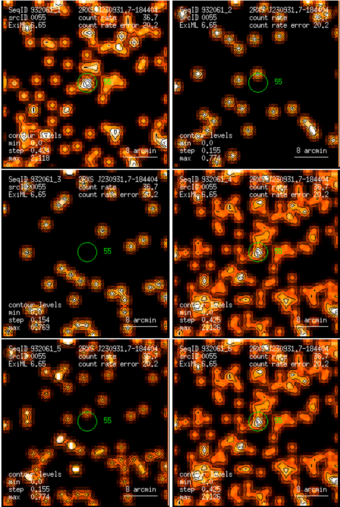
Figure 55: RASS 932061: detection 0055: band rate images, Gaussian filter: (1) PSPC channels 11 – 41, (2) 52 – 90, (3) 91 – 201, (4) 11 – 235, (5) 52 – 201, (6) 11 – 201. Broad band rates in counts/ks. Band rate contour levels in counts/ks/arcmin 2 .
