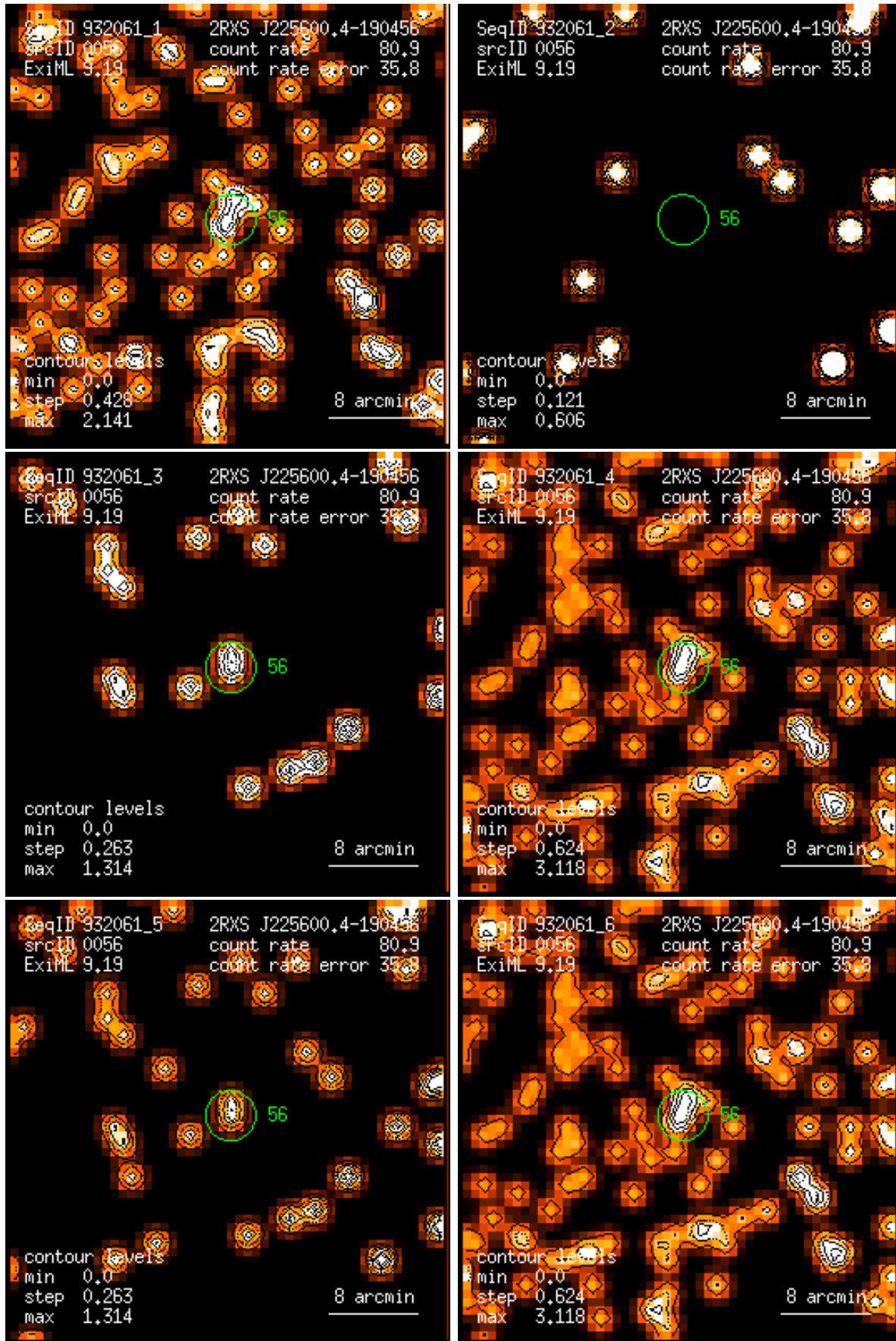
Figure 56: RASS 932061: detection 0056: band rate images, Gaussian filter: (1) PSPC channels 11 – 41, (2) 52 – 90, (3) 91 – 201, (4) 11 – 235, (5) 52 – 201, (6) 11 – 201. Broad band rates in counts/ks. Band rate contour levels in counts/ks/arcmin 2 .
