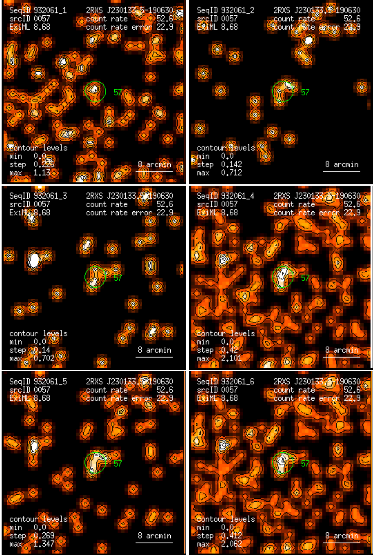
Figure 57: RASS 932061: detection 0057: band rate images, Gaussian filter: (1) PSPC channels 11 – 41, (2) 52 – 90, (3) 91 – 201, (4) 11 – 235, (5) 52 – 201, (6) 11 – 201. Broad band rates in counts/ks. Band rate contour levels in counts/ks/arcmin 2 .
