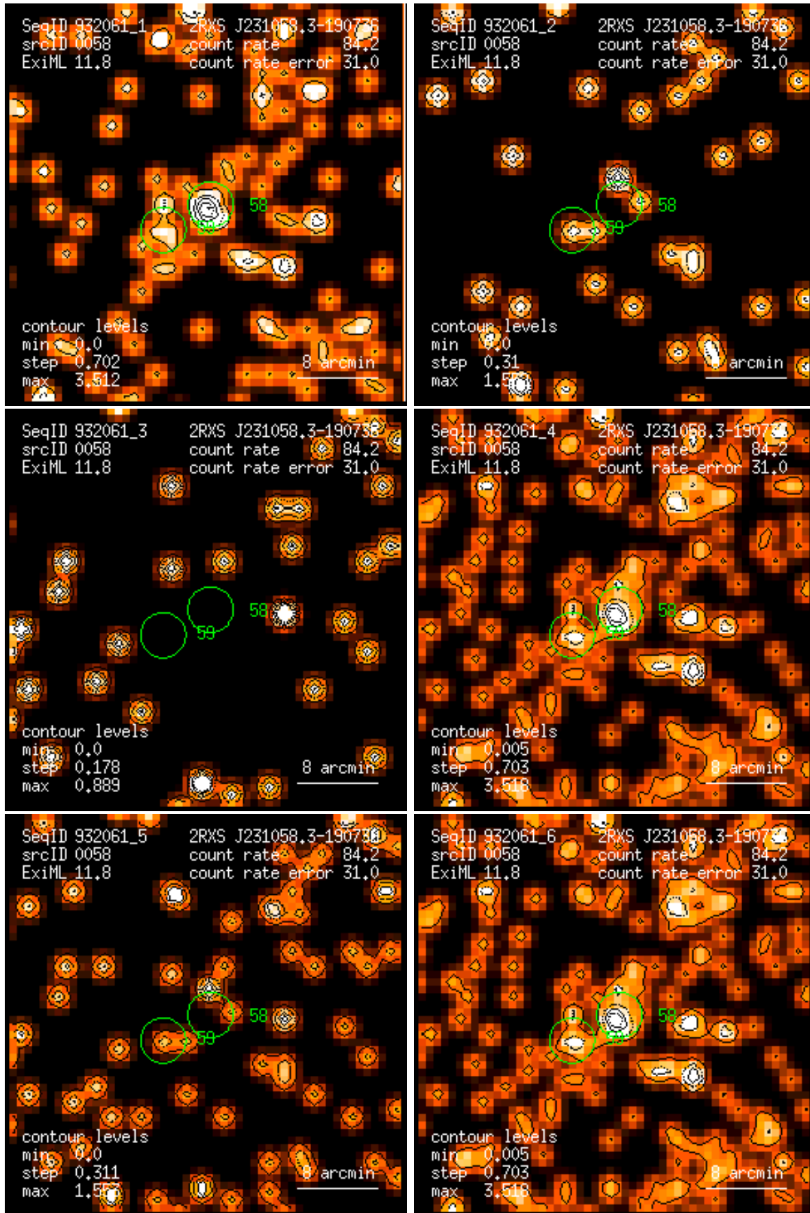
Figure 58: RASS 932061: detection 0058: band rate images, Gaussian filter: (1) PSPC channels 11 – 41, (2) 52 – 90, (3) 91 – 201, (4) 11 – 235, (5) 52 – 201, (6) 11 – 201. Broad band rates in counts/ks. Band rate contour levels in counts/ks/arcmin 2 .
