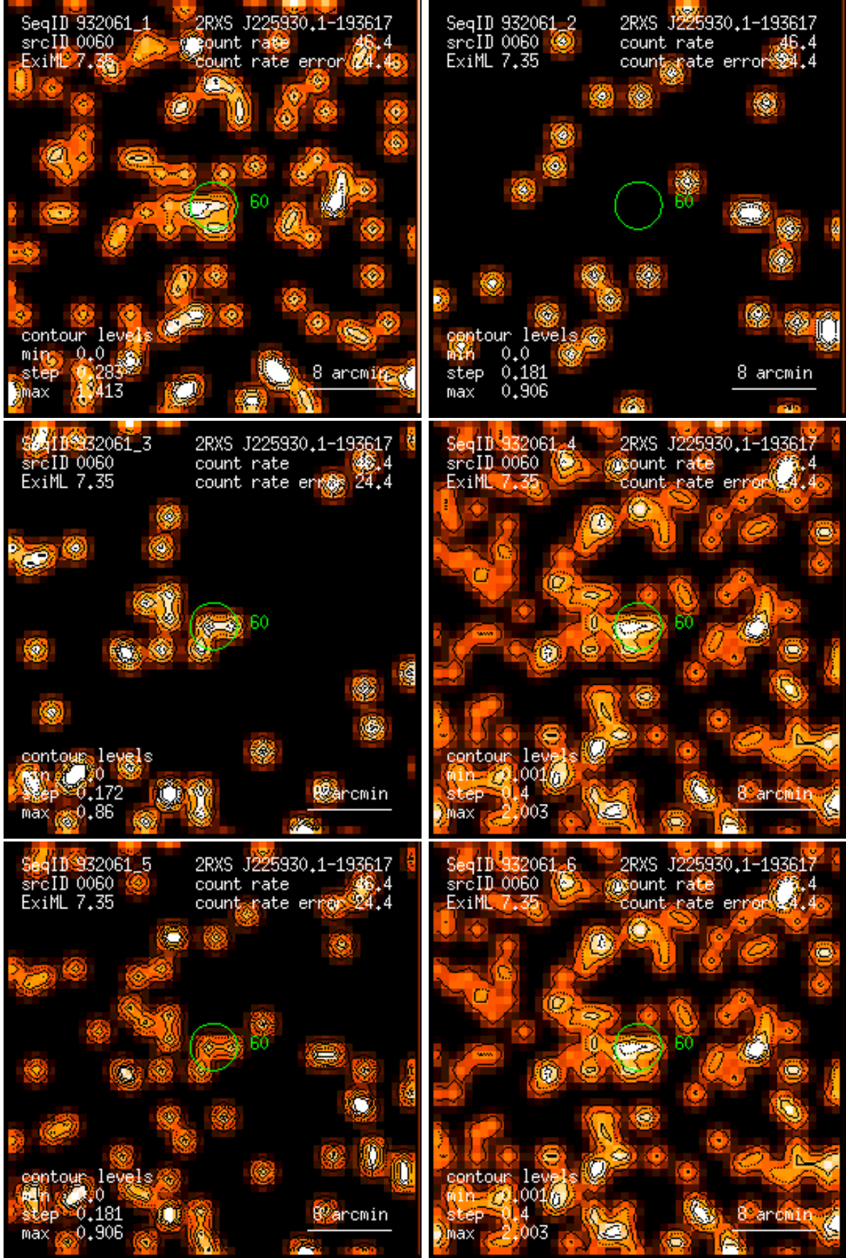
Figure 60: RASS 932061: detection 0060: band rate images, Gaussian filter: (1) PSPC channels 11 – 41, (2) 52 – 90, (3) 91 – 201, (4) 11 – 235, (5) 52 – 201, (6) 11 – 201. Broad band rates in counts/ks. Band rate contour levels in counts/ks/arcmin 2 .
