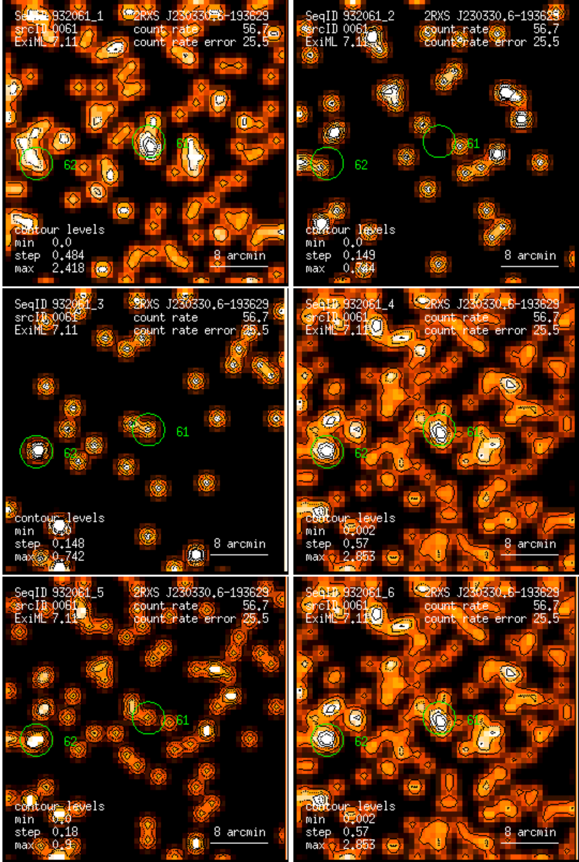
Figure 61: RASS 932061: detection 0061: band rate images, Gaussian filter: (1) PSPC channels 11 – 41, (2) 52 – 90, (3) 91 – 201, (4) 11 – 235, (5) 52 – 201, (6) 11 – 201. Broad band rates in counts/ks. Band rate contour levels in counts/ks/arcmin 2 .
