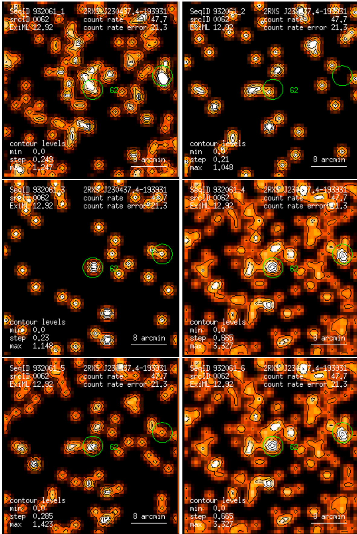
Figure 62: RASS 932061: detection 0062: band rate images, Gaussian filter: (1) PSPC channels 11 – 41, (2) 52 – 90, (3) 91 – 201, (4) 11 – 235, (5) 52 – 201, (6) 11 – 201. Broad band rates in counts/ks. Band rate contour levels in counts/ks/arcmin 2 .
