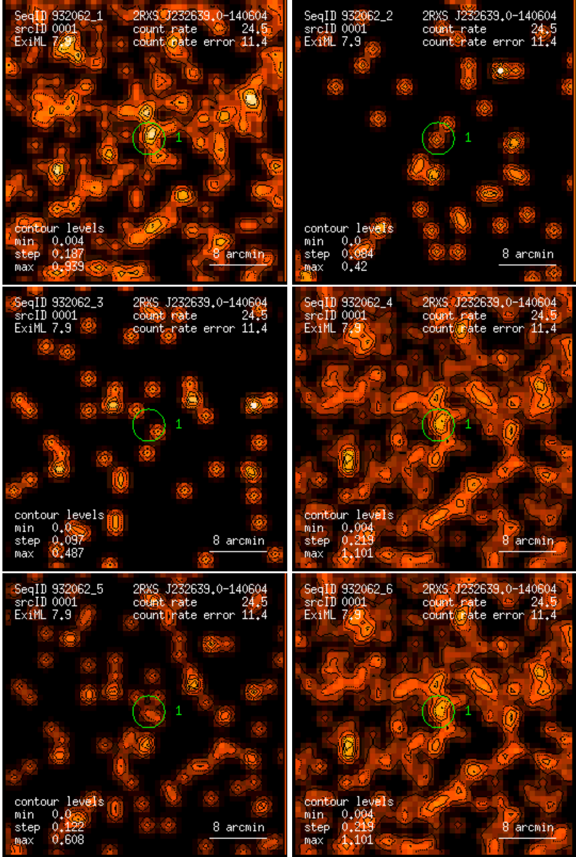
Figure 1: RASS 932062: detection 0001: band rate images, Gaussian filter: (1) PSPC channels 11 – 41, (2) 52 – 90, (3) 91 – 201, (4) 11 – 235, (5) 52 – 201, (6) 11 – 201. Broad band rates in counts/ks. Band rate contour levels in counts/ks/arcmin 2 .
