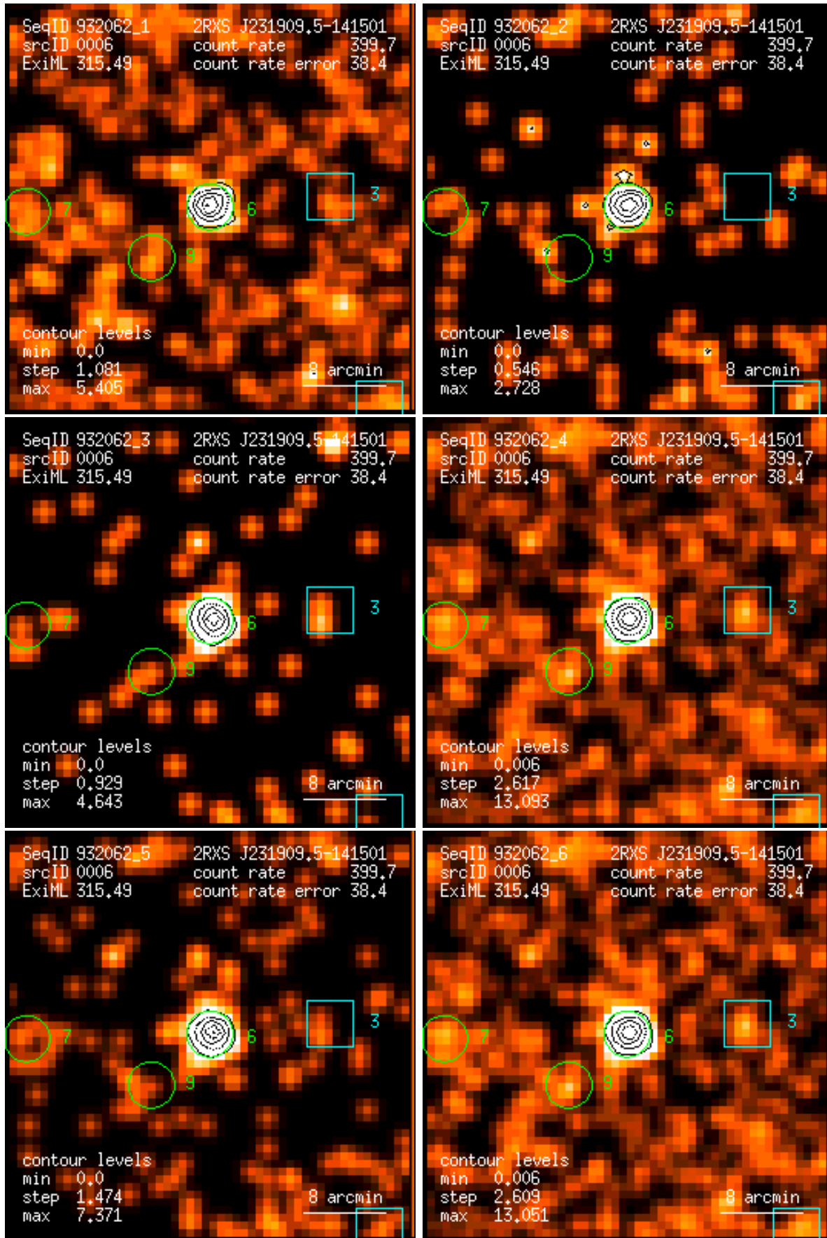
Figure 6: RASS 932062: detection 0006: band rate images, Gaussian filter: (1) PSPC channels 11 – 41, (2) 52 – 90, (3) 91 – 201, (4) 11 – 235, (5) 52 – 201, (6) 11 – 201. Broad band rates in counts/ks. Band rate contour levels in counts/ks/arcmin 2 .
