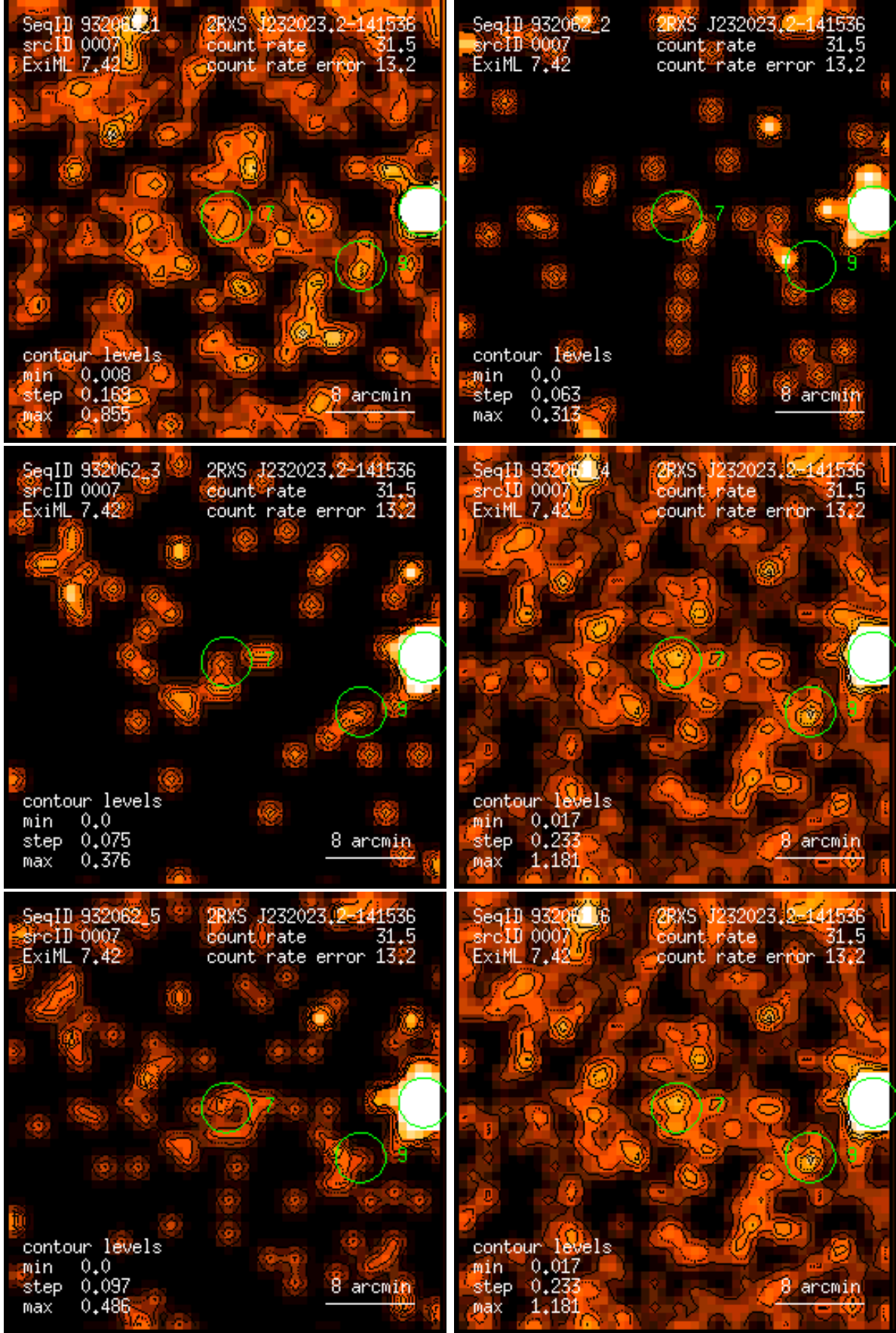
Figure 7: RASS 932062: detection 0007: band rate images, Gaussian filter: (1) PSPC channels 11 – 41, (2) 52 – 90, (3) 91 – 201, (4) 11 – 235, (5) 52 – 201, (6) 11 – 201. Broad band rates in counts/ks. Band rate contour levels in counts/ks/arcmin 2 .
