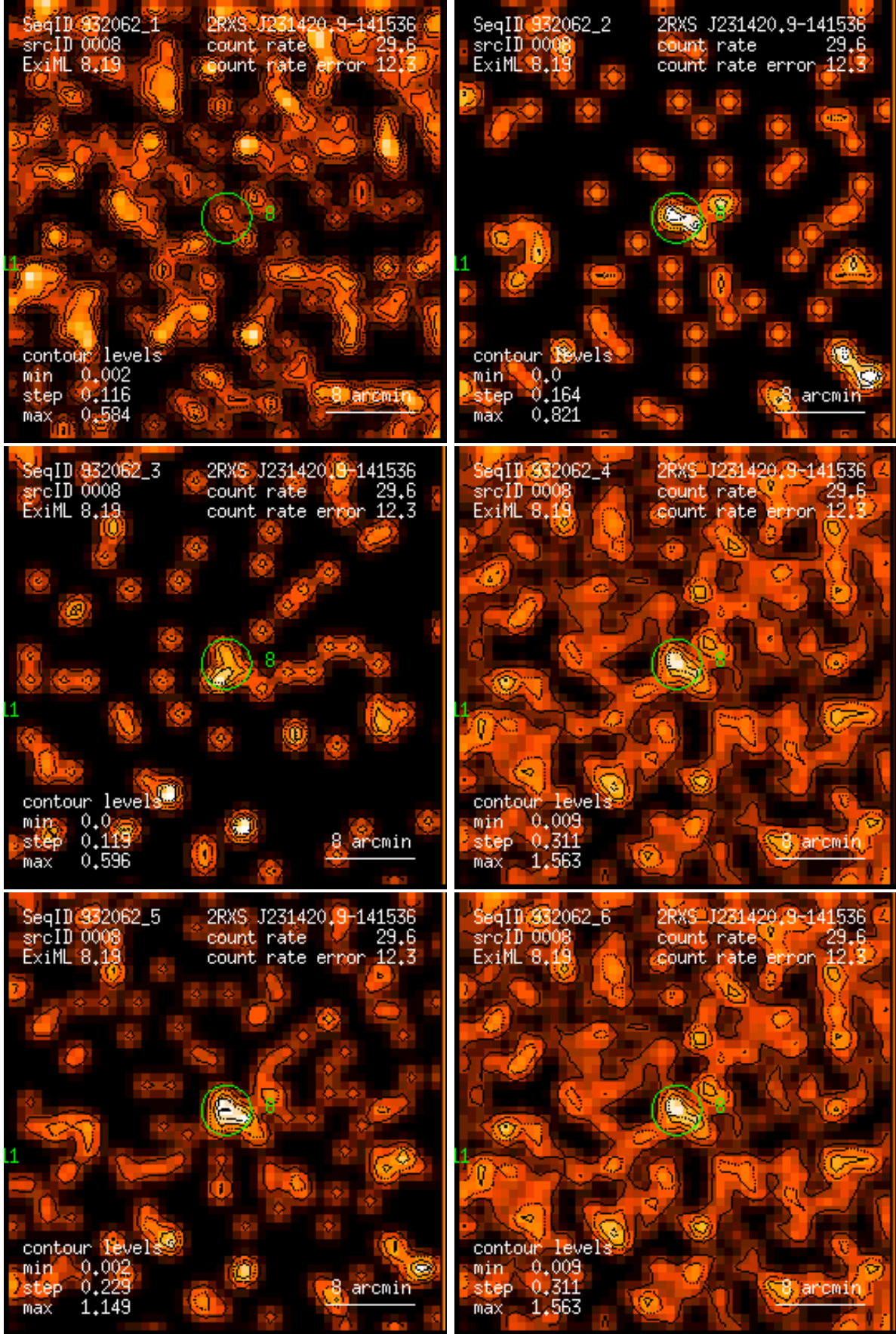
Figure 8: RASS 932062: detection 0008: band rate images, Gaussian filter: (1) PSPC channels 11 – 41, (2) 52 – 90, (3) 91 – 201, (4) 11 – 235, (5) 52 – 201, (6) 11 – 201. Broad band rates in counts/ks. Band rate contour levels in counts/ks/arcmin 2 .
