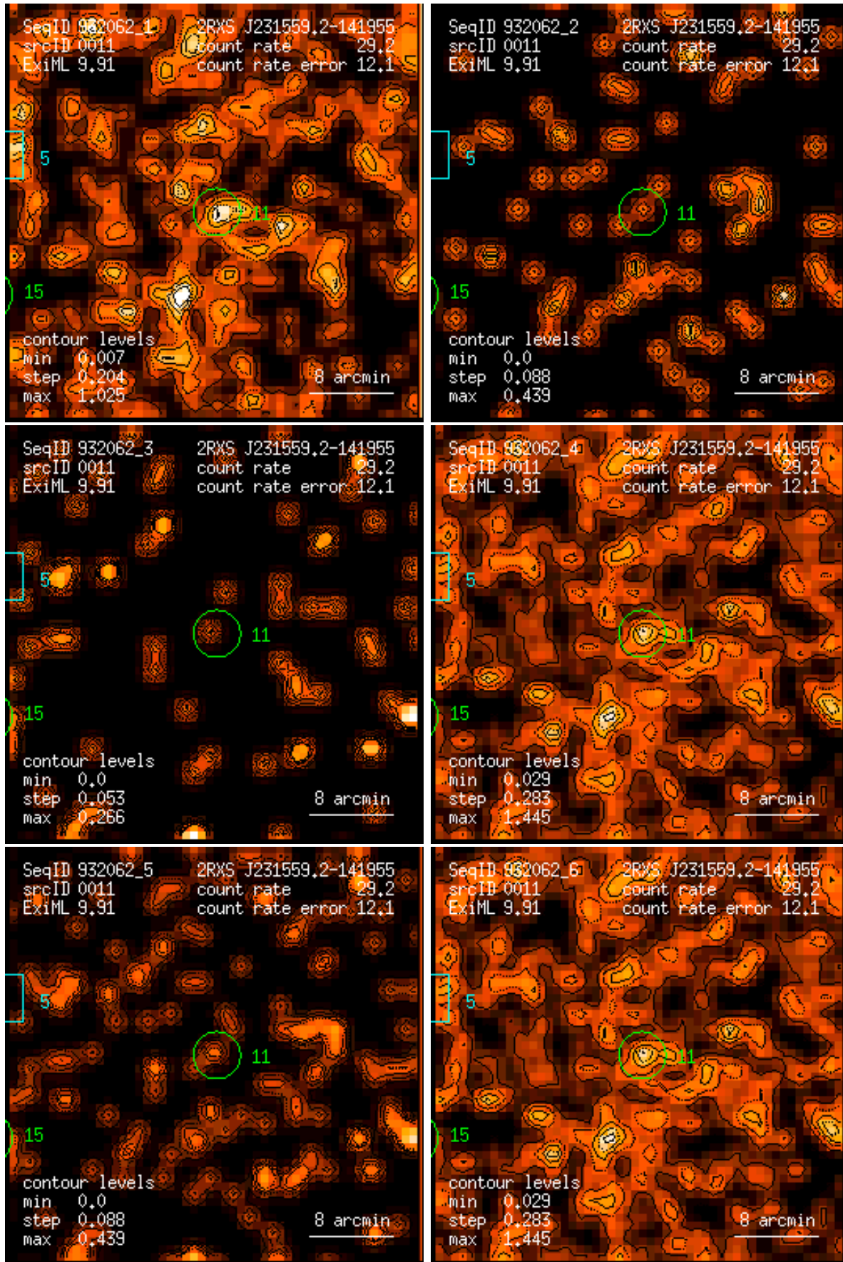
Figure 11: RASS 932062: detection 0011: band rate images, Gaussian filter: (1) PSPC channels 11 – 41, (2) 52 – 90, (3) 91 – 201, (4) 11 – 235, (5) 52 – 201, (6) 11 – 201. Broad band rates in counts/ks. Band rate contour levels in counts/ks/arcmin 2 .
