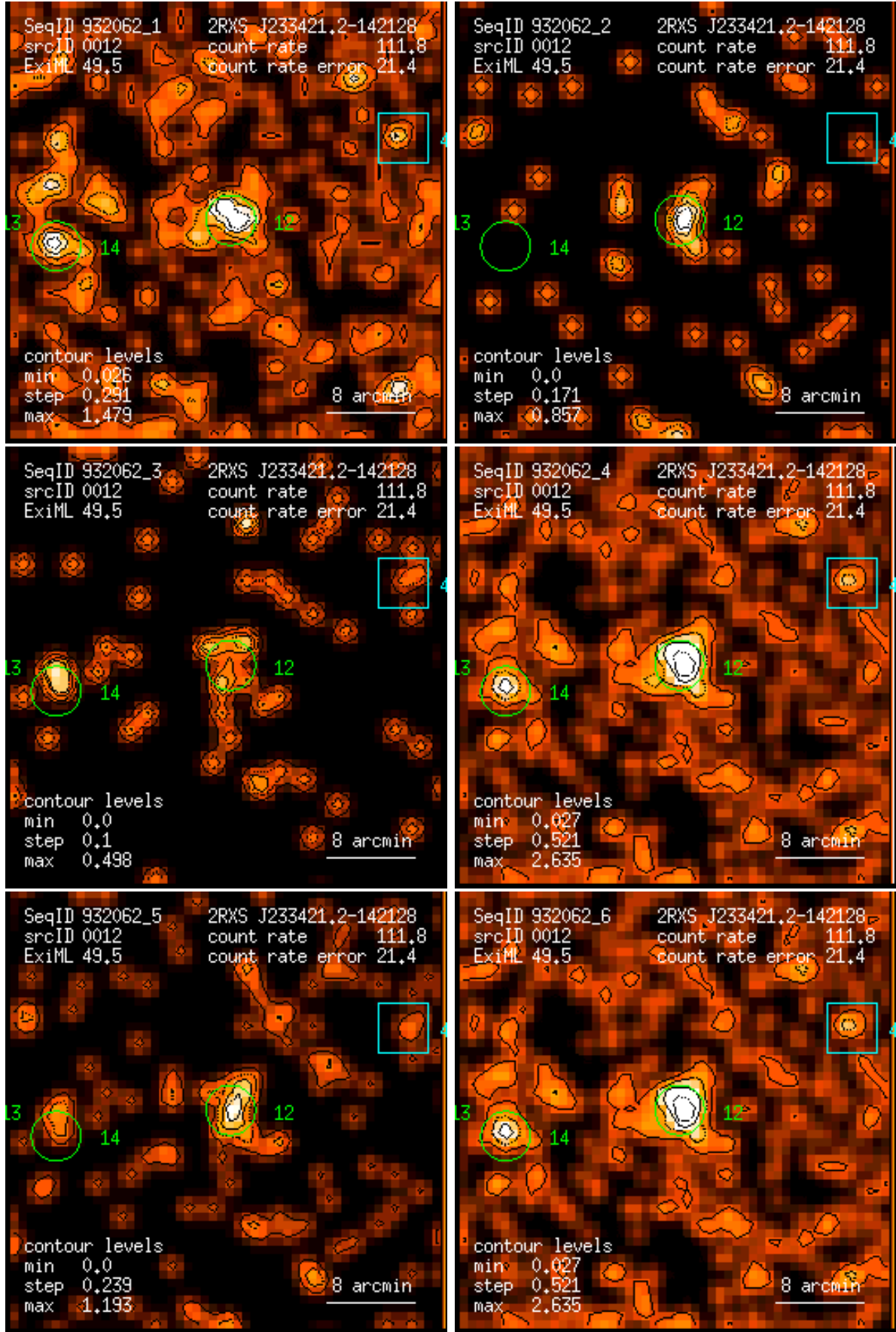
Figure 12: RASS 932062: detection 0012: band rate images, Gaussian filter: (1) PSPC channels 11 – 41, (2) 52 – 90, (3) 91 – 201, (4) 11 – 235, (5) 52 – 201, (6) 11 – 201. Broad band rates in counts/ks. Band rate contour levels in counts/ks/arcmin 2 .
