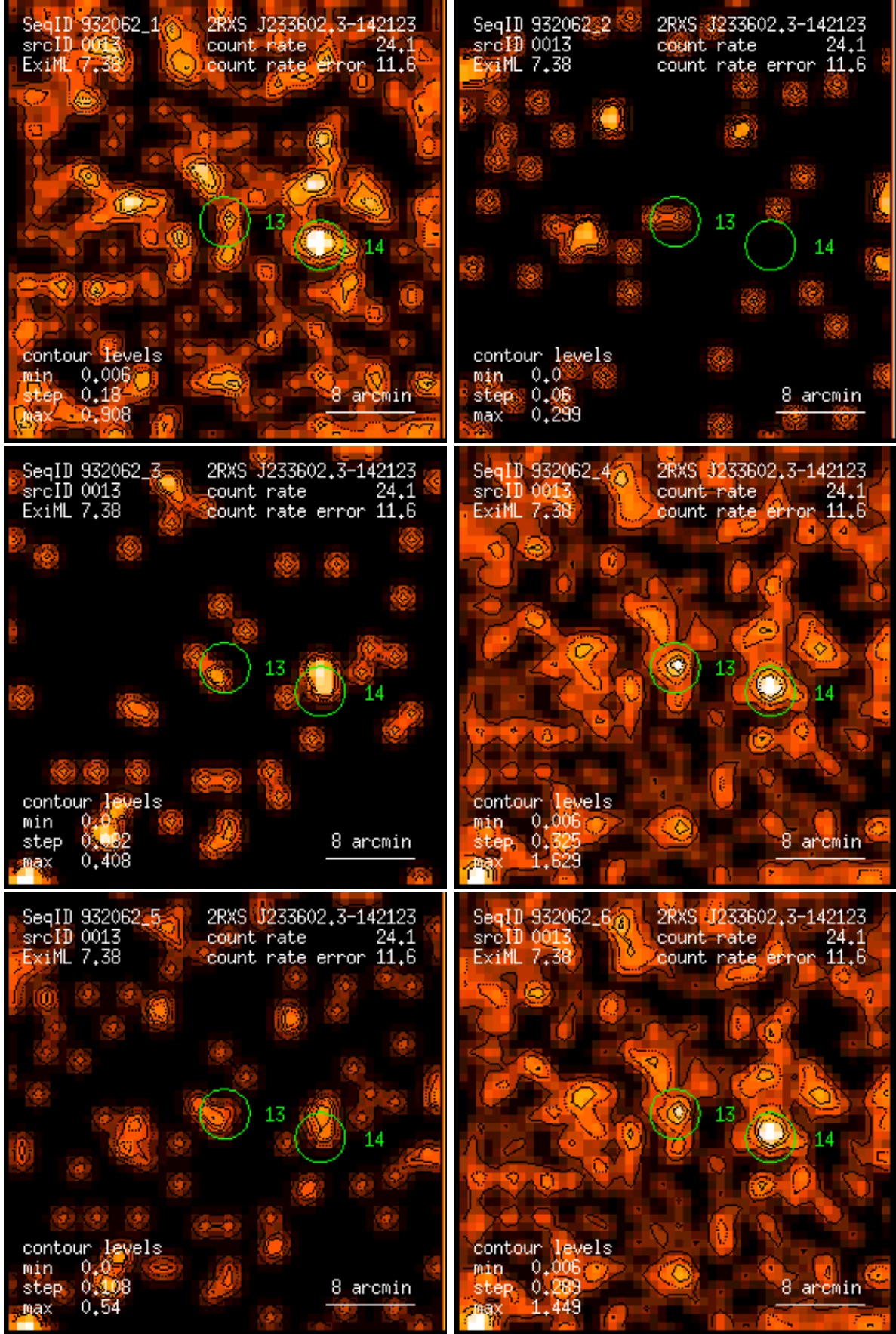
Figure 13: RASS 932062: detection 0013: band rate images, Gaussian filter: (1) PSPC channels 11 – 41, (2) 52 – 90, (3) 91 – 201, (4) 11 – 235, (5) 52 – 201, (6) 11 – 201. Broad band rates in counts/ks. Band rate contour levels in counts/ks/arcmin 2 .
