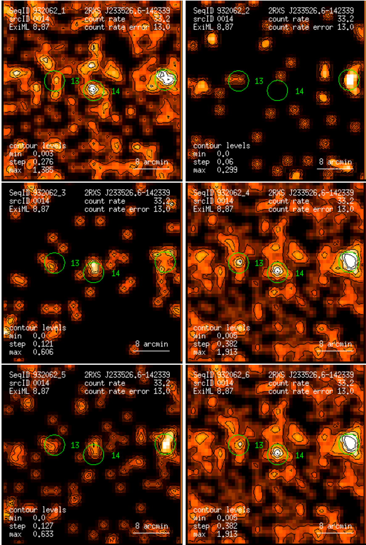
Figure 14: RASS 932062: detection 0014: band rate images, Gaussian filter: (1) PSPC channels 11 – 41, (2) 52 – 90, (3) 91 – 201, (4) 11 – 235, (5) 52 – 201, (6) 11 – 201. Broad band rates in counts/ks. Band rate contour levels in counts/ks/arcmin 2 .
