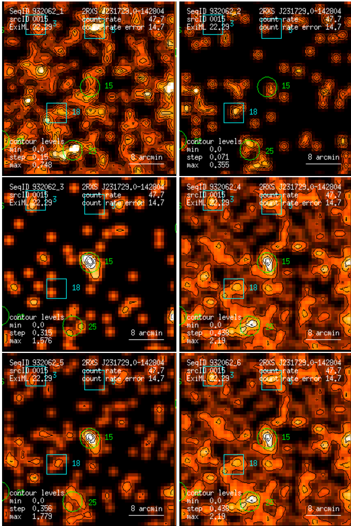
Figure 15: RASS 932062: detection 0015: band rate images, Gaussian filter: (1) PSPC channels 11 – 41, (2) 52 – 90, (3) 91 – 201, (4) 11 – 235, (5) 52 – 201, (6) 11 – 201. Broad band rates in counts/ks. Band rate contour levels in counts/ks/arcmin 2 .
