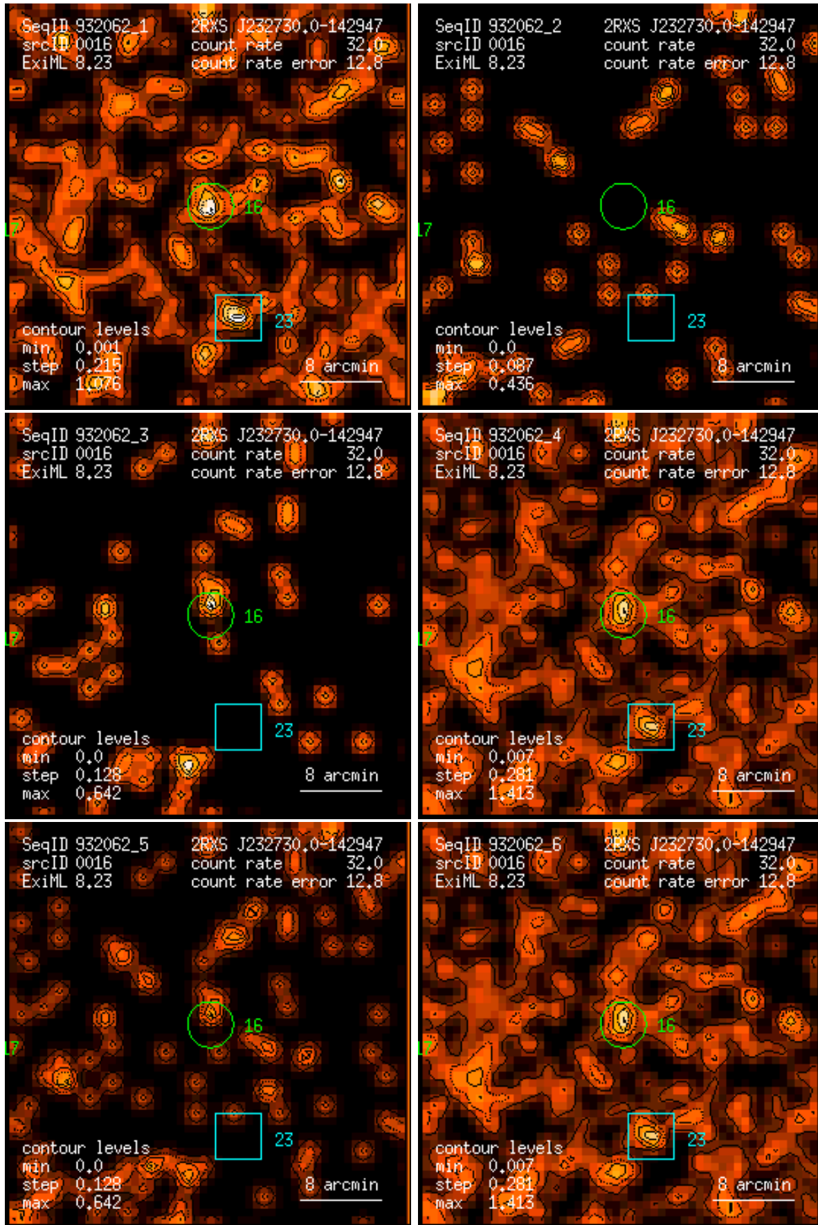
Figure 16: RASS 932062: detection 0016: band rate images, Gaussian filter: (1) PSPC channels 11 – 41, (2) 52 – 90, (3) 91 – 201, (4) 11 – 235, (5) 52 – 201, (6) 11 – 201. Broad band rates in counts/ks. Band rate contour levels in counts/ks/arcmin 2 .
