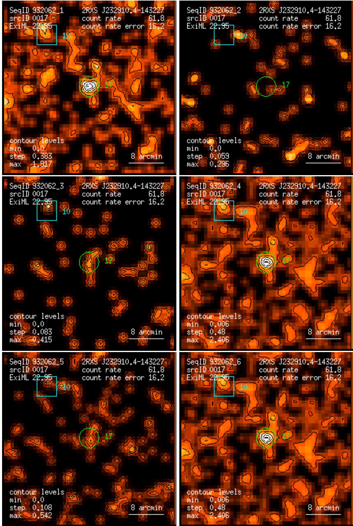
Figure 17: RASS 932062: detection 0017: band rate images, Gaussian filter: (1) PSPC channels 11 – 41, (2) 52 – 90, (3) 91 – 201, (4) 11 – 235, (5) 52 – 201, (6) 11 – 201. Broad band rates in counts/ks. Band rate contour levels in counts/ks/arcmin 2 .
