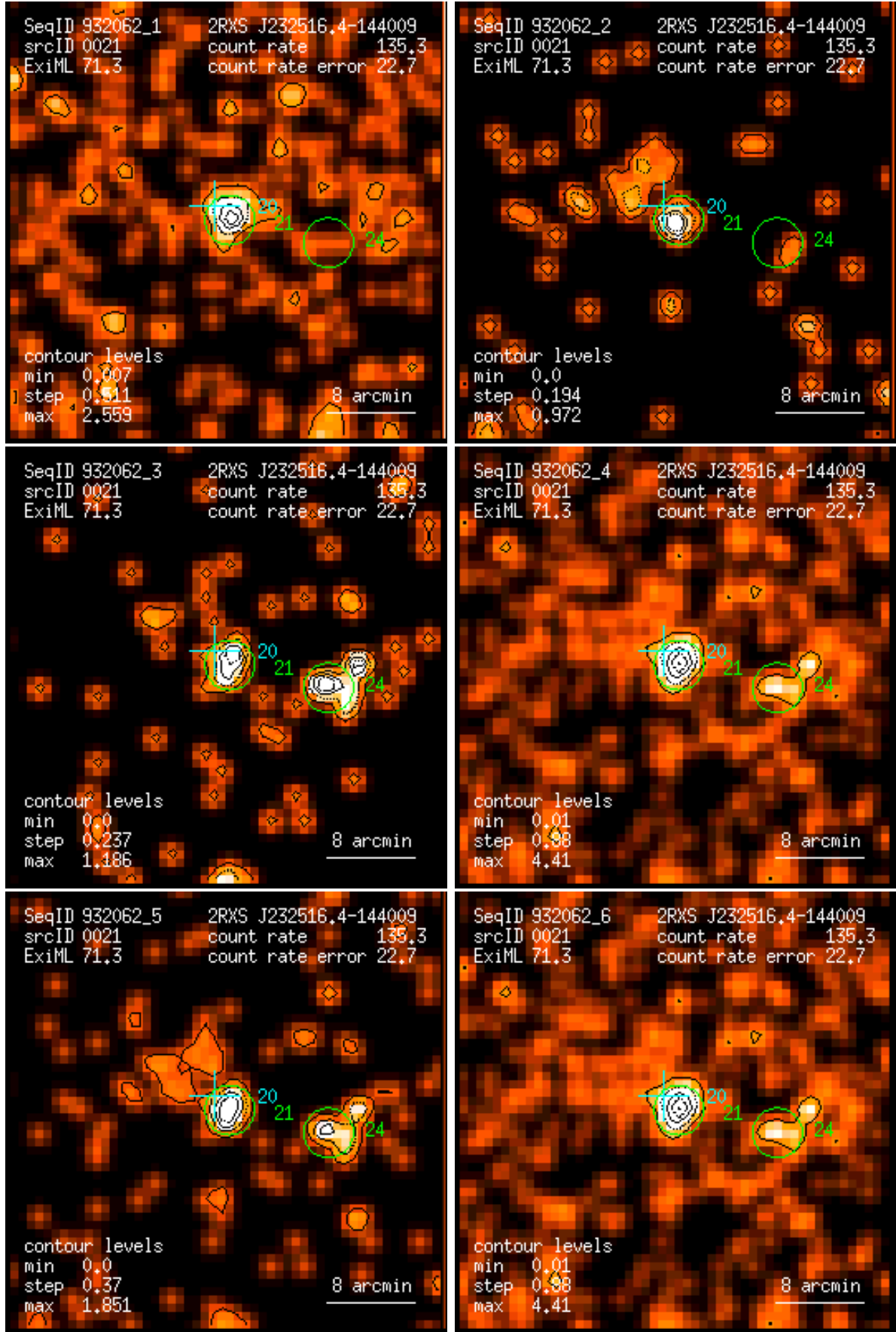
Figure 21: RASS 932062: detection 0021: band rate images, Gaussian filter: (1) PSPC channels 11 – 41, (2) 52 – 90, (3) 91 – 201, (4) 11 – 235, (5) 52 – 201, (6) 11 – 201. Broad band rates in counts/ks. Band rate contour levels in counts/ks/arcmin 2 .
