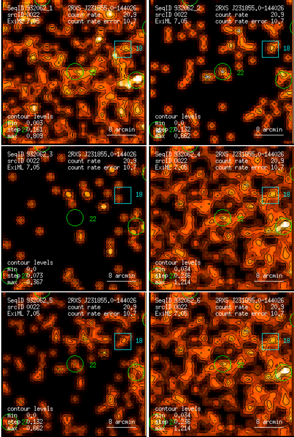
Figure 22: RASS 932062: detection 0022: band rate images, Gaussian filter: (1) PSPC channels 11 – 41, (2) 52 – 90, (3) 91 – 201, (4) 11 – 235, (5) 52 – 201, (6) 11 – 201. Broad band rates in counts/ks. Band rate contour levels in counts/ks/arcmin 2 .
