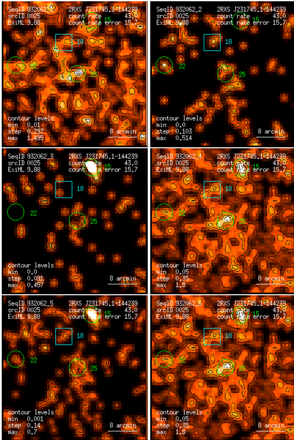
Figure 25: RASS 932062: detection 0025: band rate images, Gaussian filter: (1) PSPC channels 11 – 41, (2) 52 – 90, (3) 91 – 201, (4) 11 – 235, (5) 52 – 201, (6) 11 – 201. Broad band rates in counts/ks. Band rate contour levels in counts/ks/arcmin 2 .
